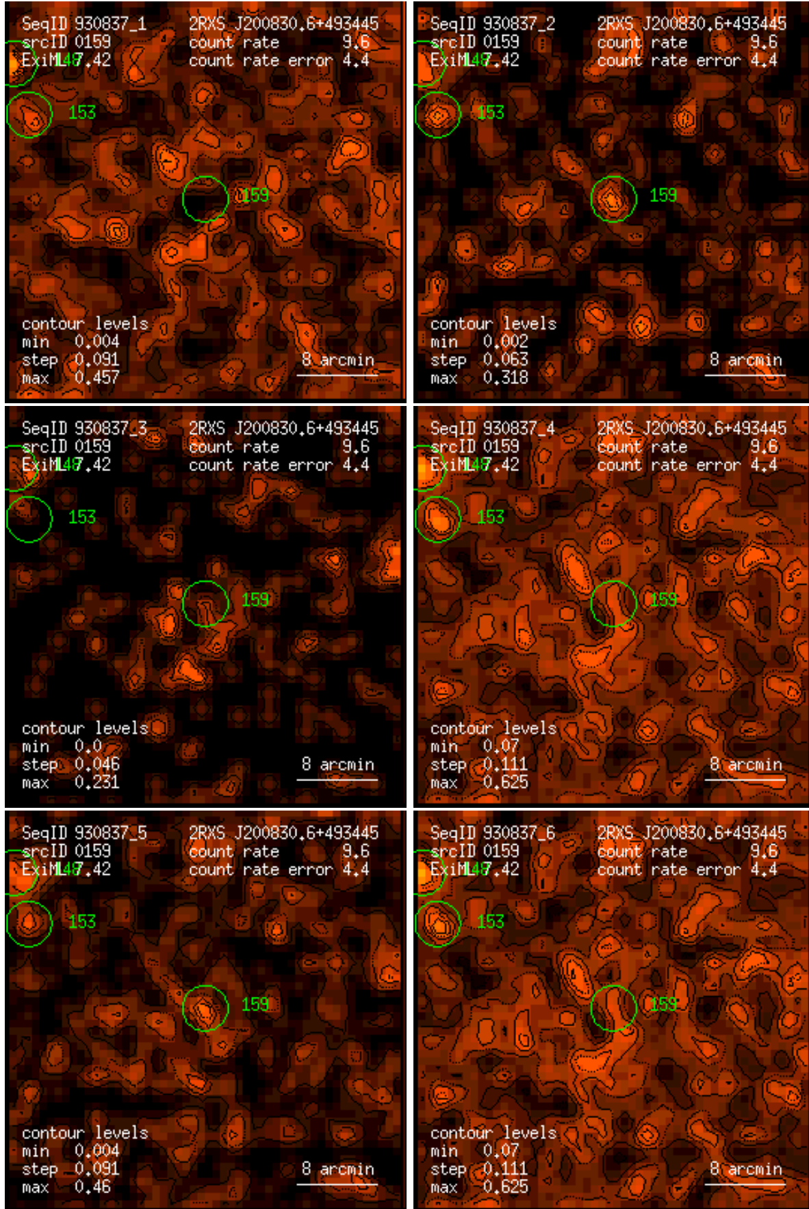
Figure 159: RASS 930837: detection 0159: band rate images, Gaussian filter: (1) PSPC channels 11 – 41, (2) 52 – 90, (3) 91 – 201, (4) 11 – 235, (5) 52 – 201, (6) 11 – 201. Broad band rates in counts/ks. Band rate contour levels in counts/ks/arcmin 2 .
