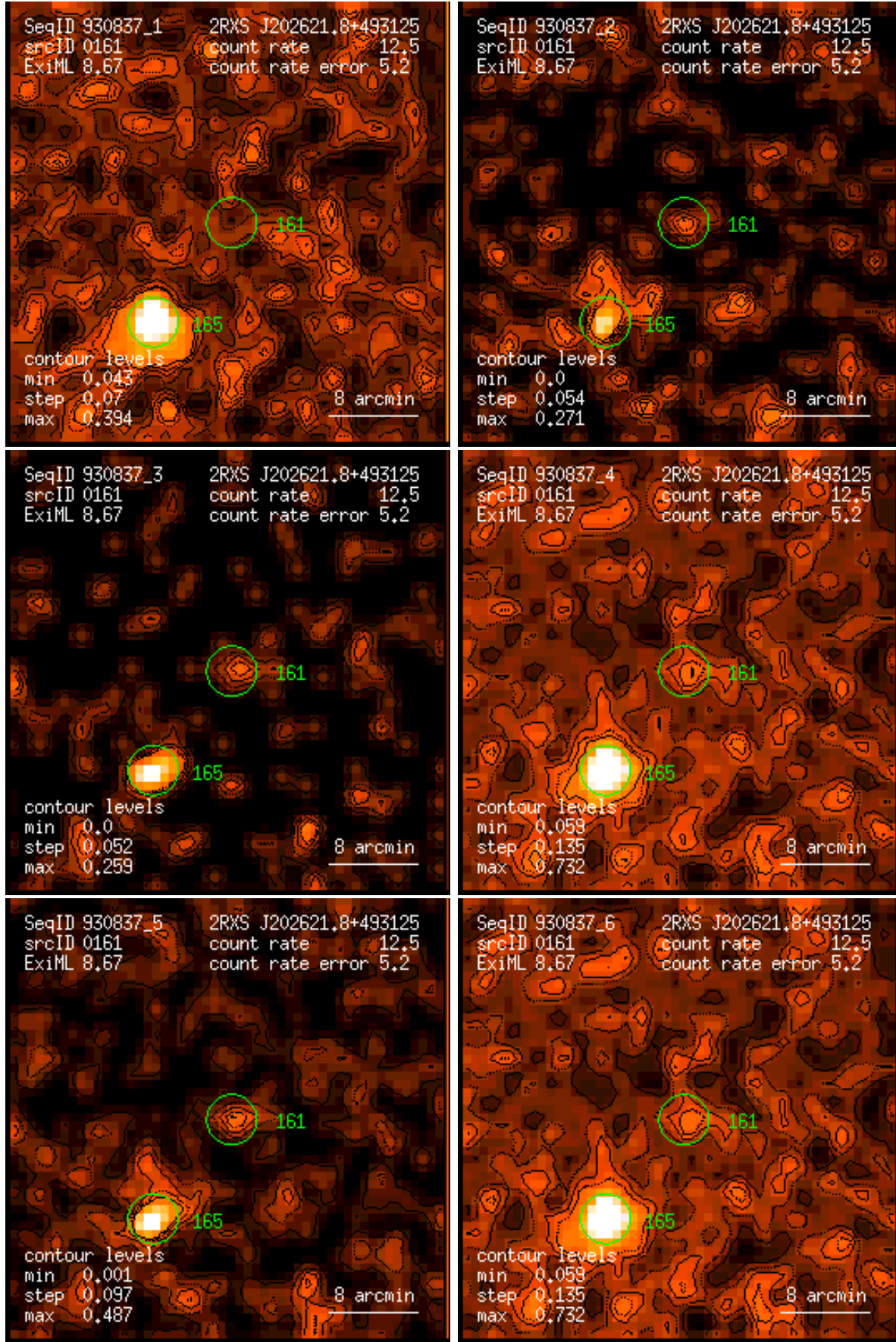
Figure 161: RASS 930837: detection 0161: band rate images, Gaussian filter: (1) PSPC channels 11 – 41, (2) 52 – 90, (3) 91 – 201, (4) 11 – 235, (5) 52 – 201, (6) 11 – 201. Broad band rates in counts/ks. Band rate contour levels in counts/ks/arcmin 2 .
