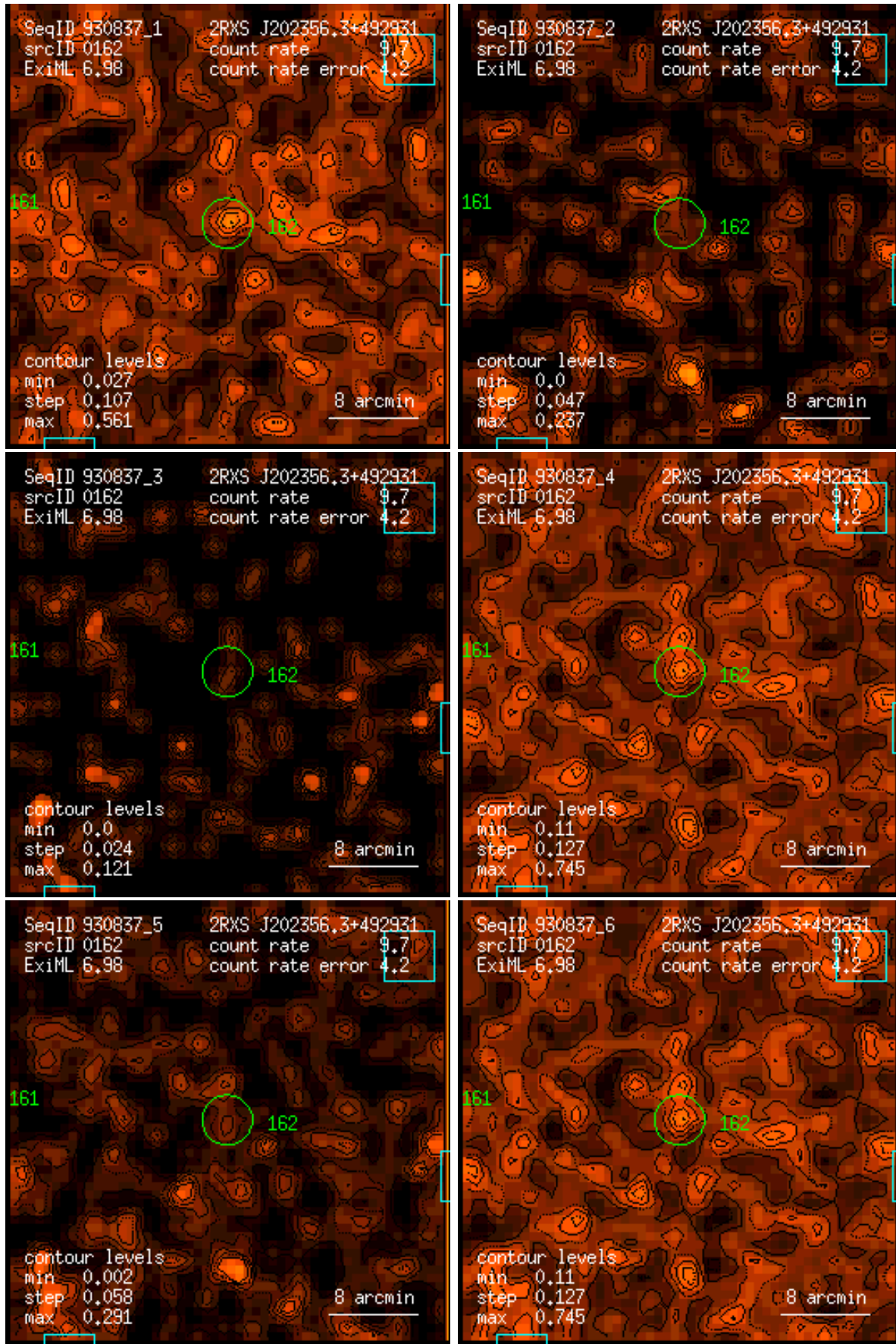
Figure 162: RASS 930837: detection 0162: band rate images, Gaussian filter: (1) PSPC channels 11 – 41, (2) 52 – 90, (3) 91 – 201, (4) 11 – 235, (5) 52 – 201, (6) 11 – 201. Broad band rates in counts/ks. Band rate contour levels in counts/ks/arcmin 2 .
