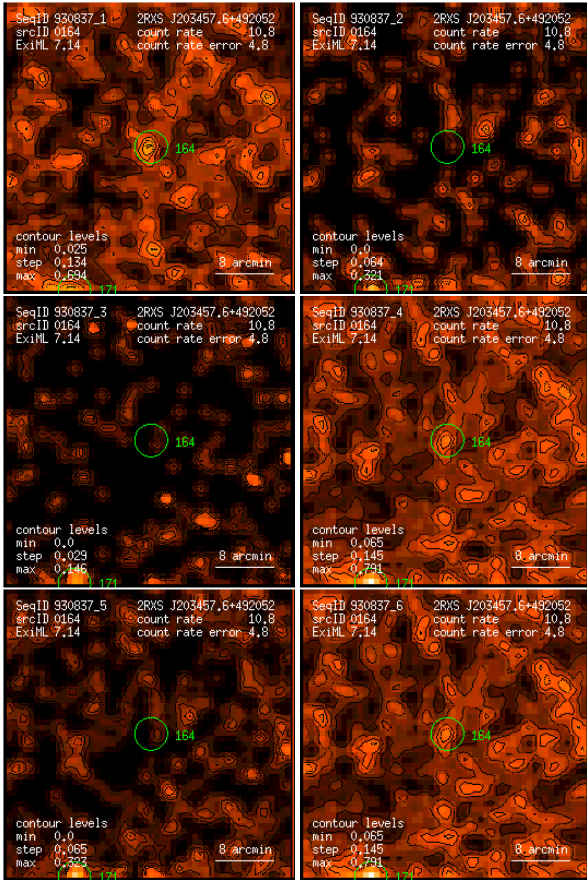
Figure 164: RASS 930837: detection 0164: band rate images, Gaussian filter: (1) PSPC channels 11 – 41, (2) 52 – 90, (3) 91 – 201, (4) 11 – 235, (5) 52 – 201, (6) 11 – 201. Broad band rates in counts/ks. Band rate contour levels in counts/ks/arcmin 2 .
