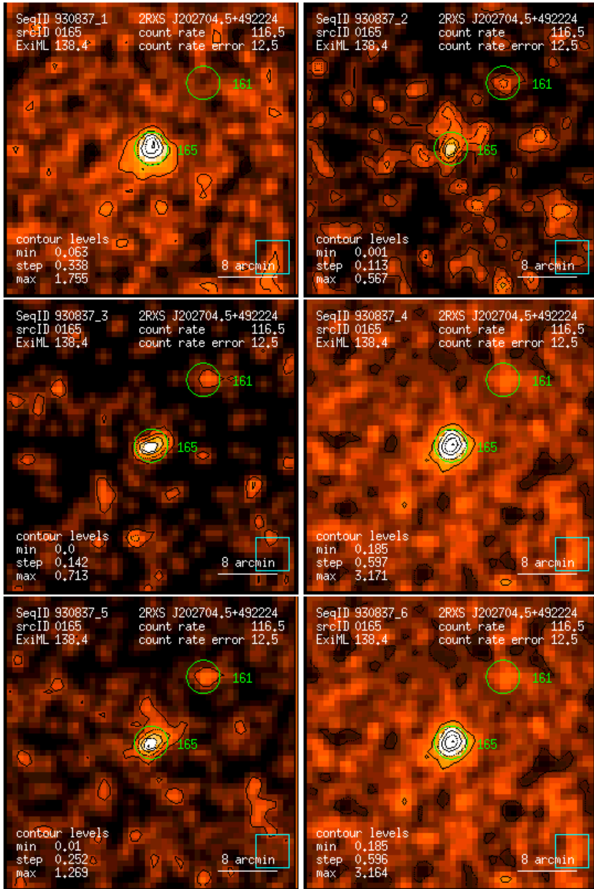
Figure 165: RASS 930837: detection 0165: band rate images, Gaussian filter: (1) PSPC channels 11 – 41, (2) 52 – 90, (3) 91 – 201, (4) 11 – 235, (5) 52 – 201, (6) 11 – 201. Broad band rates in counts/ks. Band rate contour levels in counts/ks/arcmin 2 .
