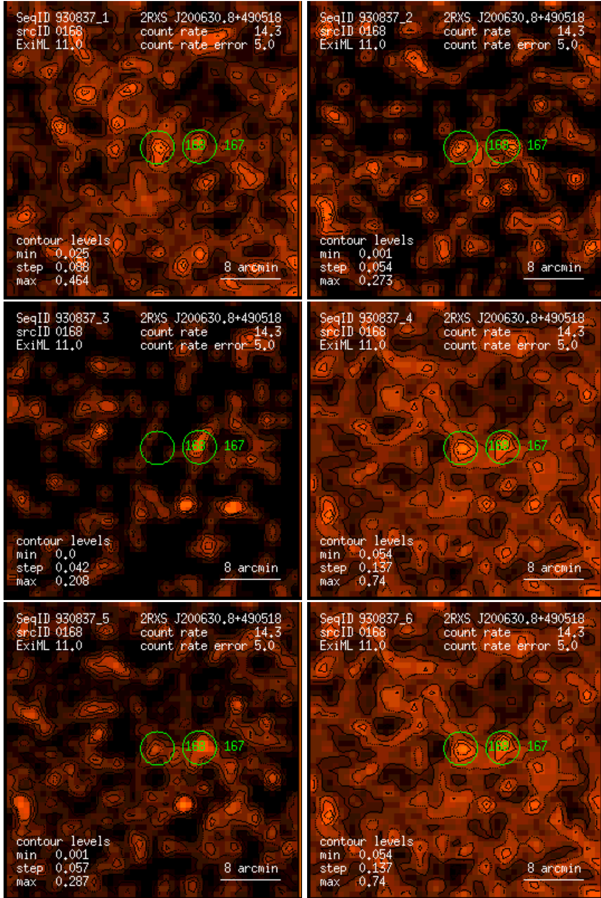
Figure 168: RASS 930837: detection 0168: band rate images, Gaussian filter: (1) PSPC channels 11 – 41, (2) 52 – 90, (3) 91 – 201, (4) 11 – 235, (5) 52 – 201, (6) 11 – 201. Broad band rates in counts/ks. Band rate contour levels in counts/ks/arcmin 2 .
