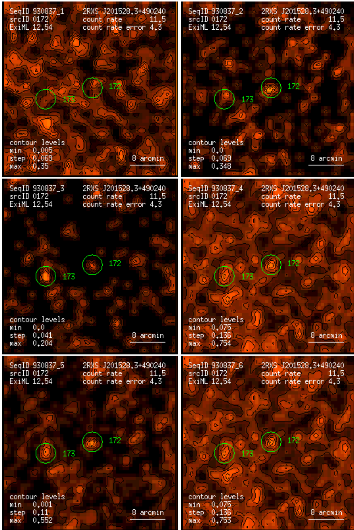
Figure 172: RASS 930837: detection 0172: band rate images, Gaussian filter: (1) PSPC channels 11 – 41, (2) 52 – 90, (3) 91 – 201, (4) 11 – 235, (5) 52 – 201, (6) 11 – 201. Broad band rates in counts/ks. Band rate contour levels in counts/ks/arcmin 2 .
