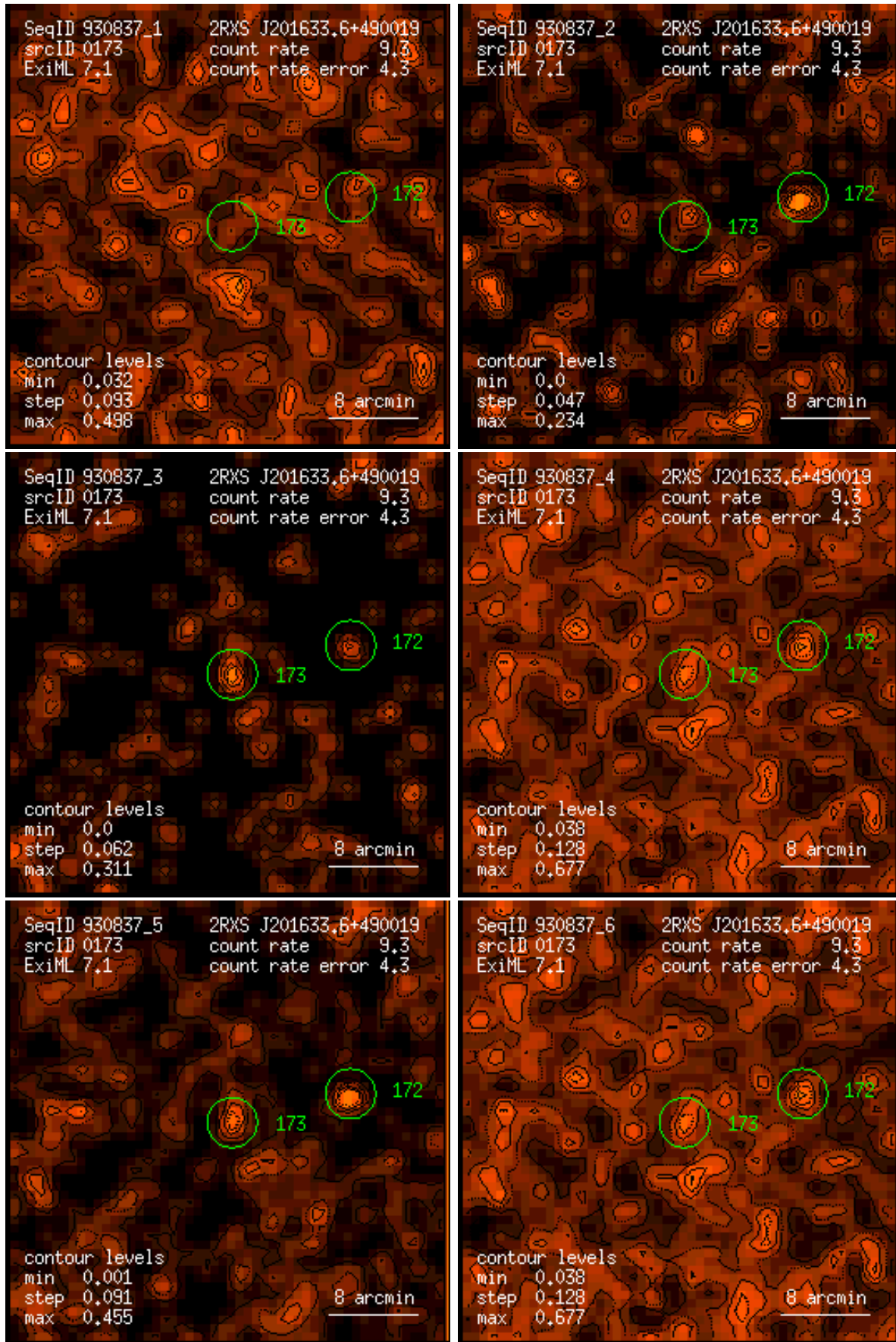
Figure 173: RASS 930837: detection 0173: band rate images, Gaussian filter: (1) PSPC channels 11 – 41, (2) 52 – 90, (3) 91 – 201, (4) 11 – 235, (5) 52 – 201, (6) 11 – 201. Broad band rates in counts/ks. Band rate contour levels in counts/ks/arcmin 2 .
