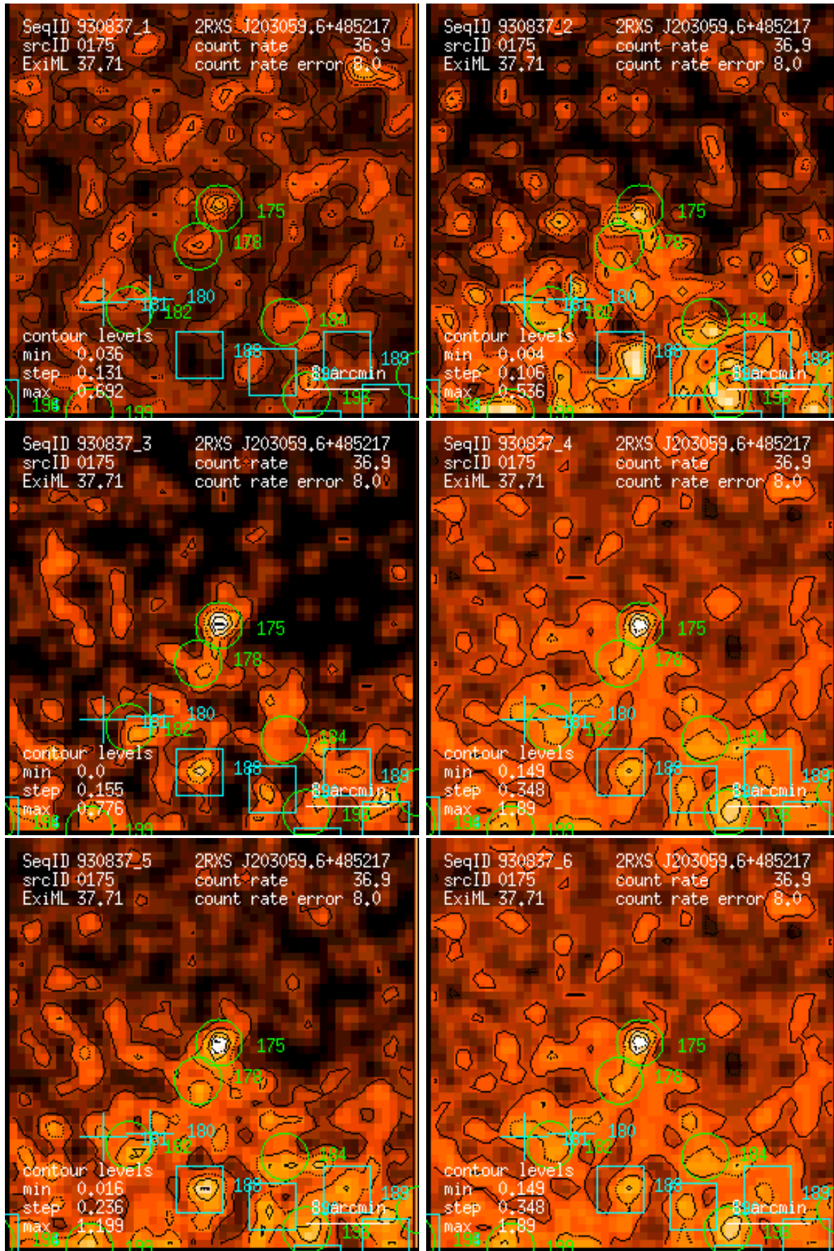
Figure 175: RASS 930837: detection 0175: band rate images, Gaussian filter: (1) PSPC channels 11 – 41, (2) 52 – 90, (3) 91 – 201, (4) 11 – 235, (5) 52 – 201, (6) 11 – 201. Broad band rates in counts/ks. Band rate contour levels in counts/ks/arcmin 2 .
