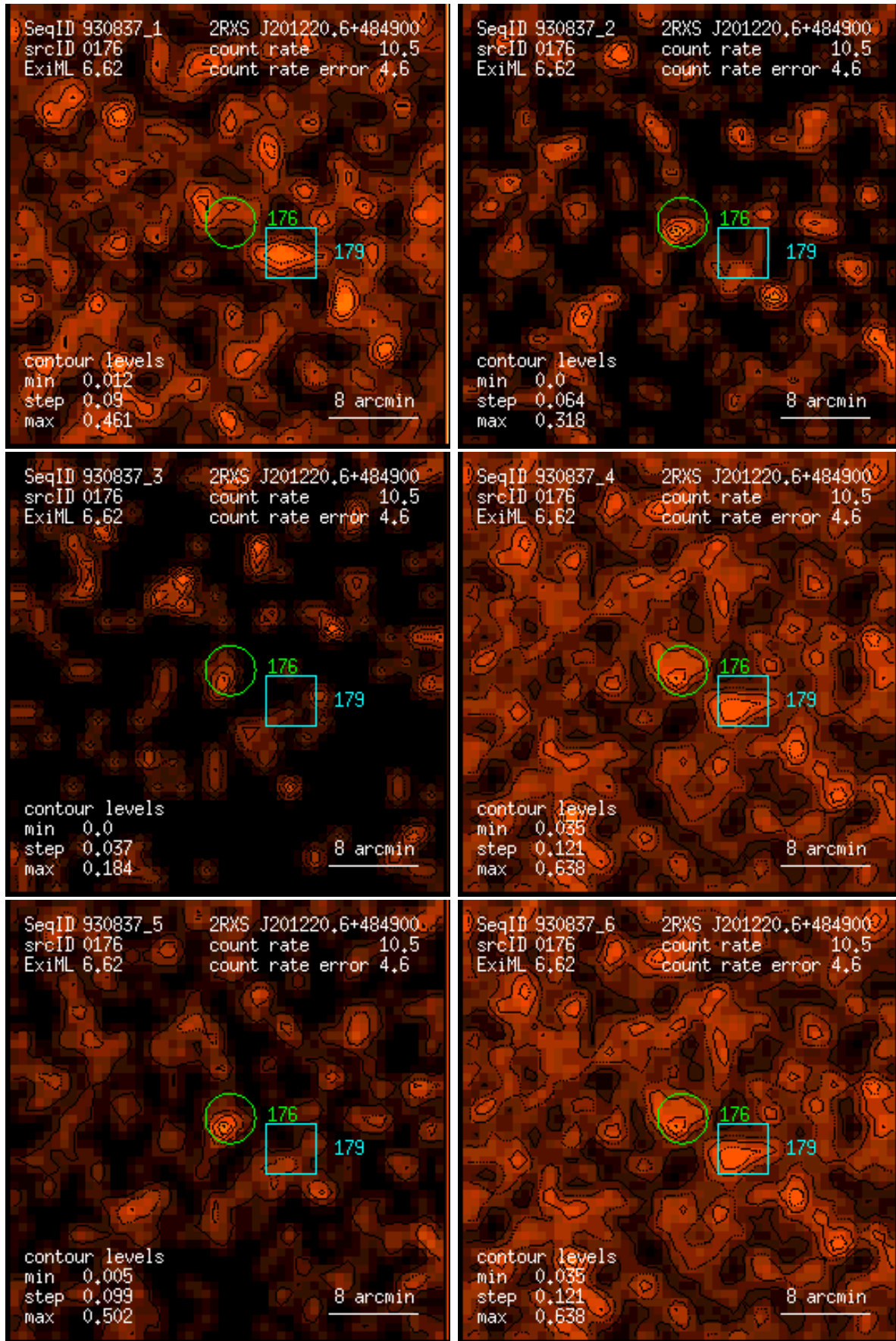
Figure 176: RASS 930837: detection 0176: band rate images, Gaussian filter: (1) PSPC channels 11 – 41, (2) 52 – 90, (3) 91 – 201, (4) 11 – 235, (5) 52 – 201, (6) 11 – 201. Broad band rates in counts/ks. Band rate contour levels in counts/ks/arcmin 2 .
