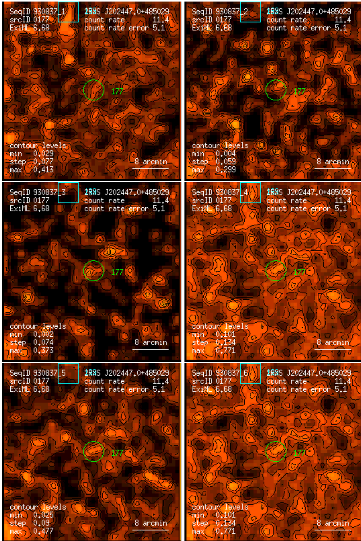
Figure 177: RASS 930837: detection 0177: band rate images, Gaussian filter: (1) PSPC channels 11 – 41, (2) 52 – 90, (3) 91 – 201, (4) 11 – 235, (5) 52 – 201, (6) 11 – 201. Broad band rates in counts/ks. Band rate contour levels in counts/ks/arcmin 2 .
