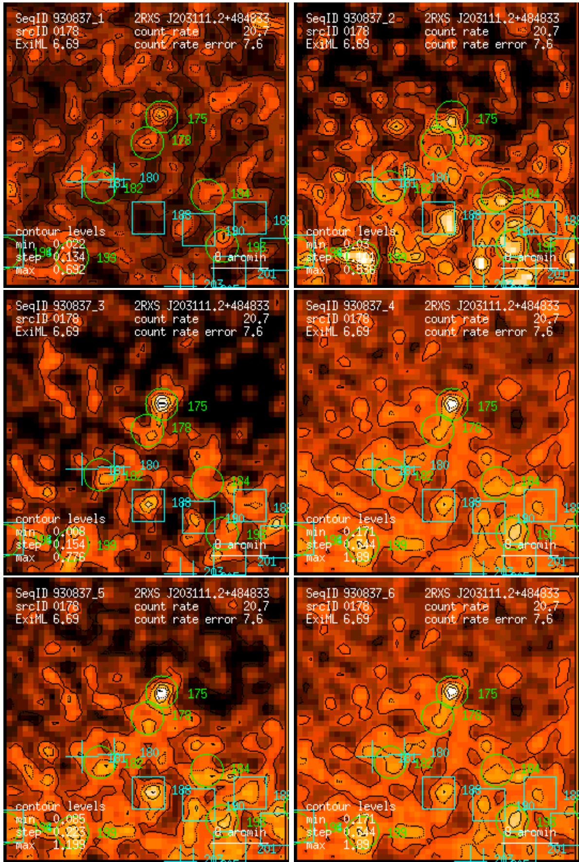
Figure 178: RASS 930837: detection 0178: band rate images, Gaussian filter: (1) PSPC channels 11 – 41, (2) 52 – 90, (3) 91 – 201, (4) 11 – 235, (5) 52 – 201, (6) 11 – 201. Broad band rates in counts/ks. Band rate contour levels in counts/ks/arcmin 2 .
