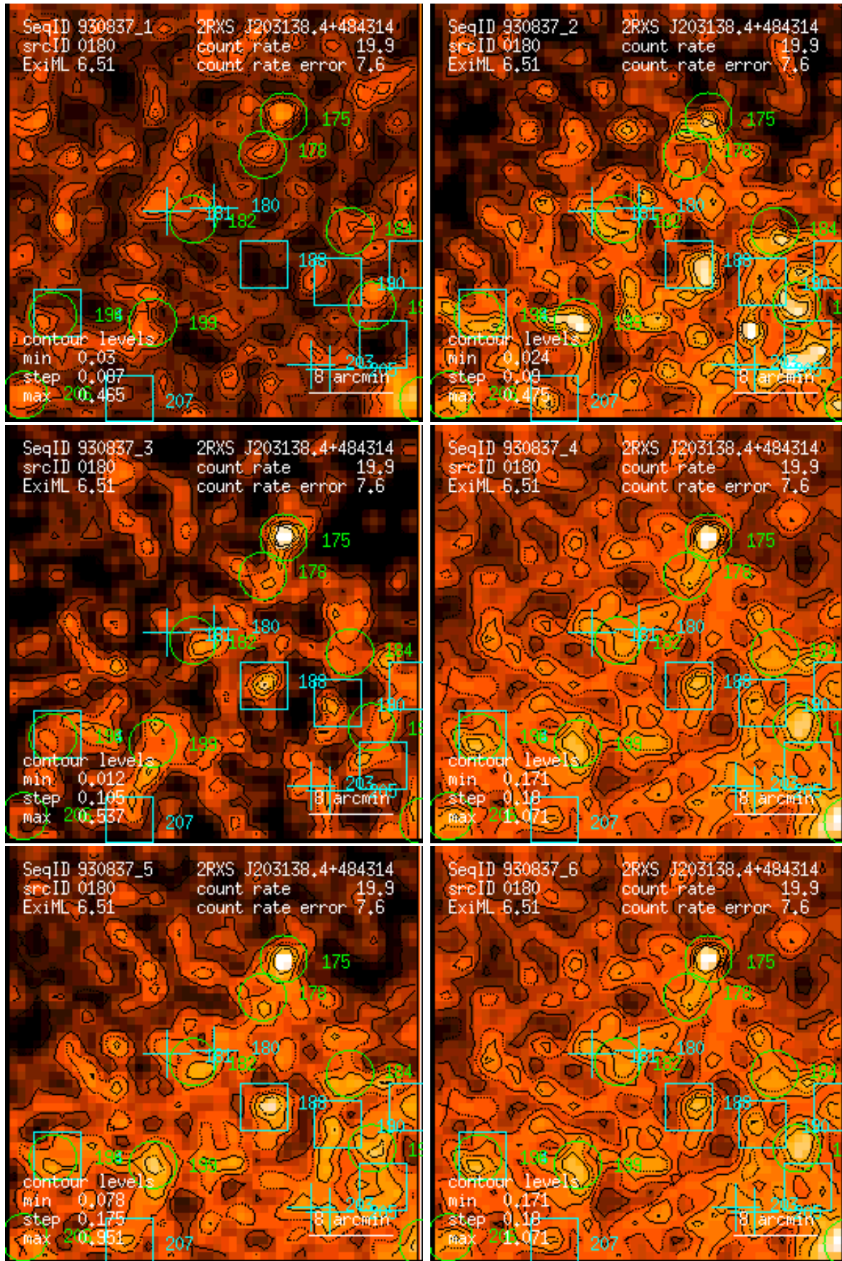
Figure 180: RASS 930837: detection 0180: band rate images, Gaussian filter: (1) PSPC channels 11 – 41, (2) 52 – 90, (3) 91 – 201, (4) 11 – 235, (5) 52 – 201, (6) 11 – 201. Broad band rates in counts/ks. Band rate contour levels in counts/ks/arcmin 2 .
