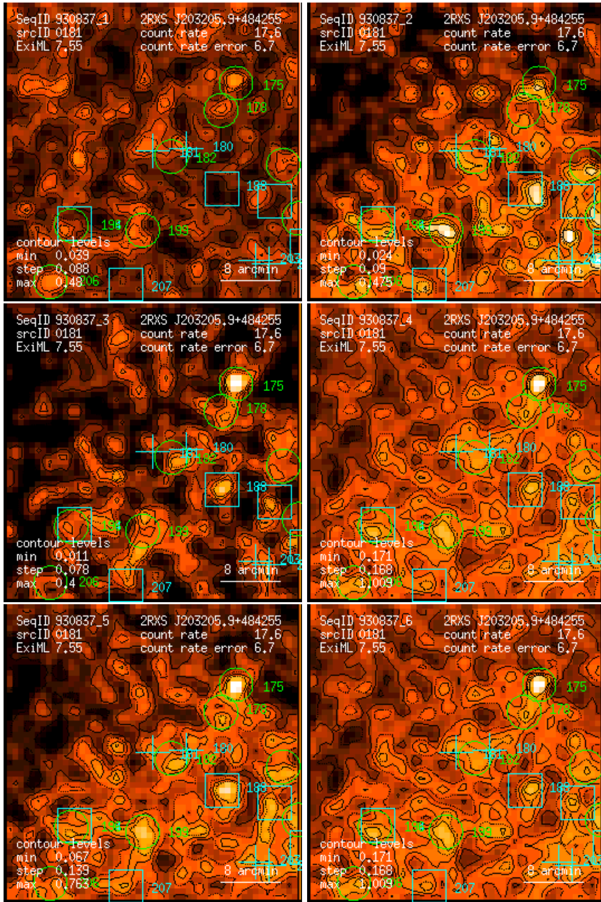
Figure 181: RASS 930837: detection 0181: band rate images, Gaussian filter: (1) PSPC channels 11 – 41, (2) 52 – 90, (3) 91 – 201, (4) 11 – 235, (5) 52 – 201, (6) 11 – 201. Broad band rates in counts/ks. Band rate contour levels in counts/ks/arcmin 2 .
