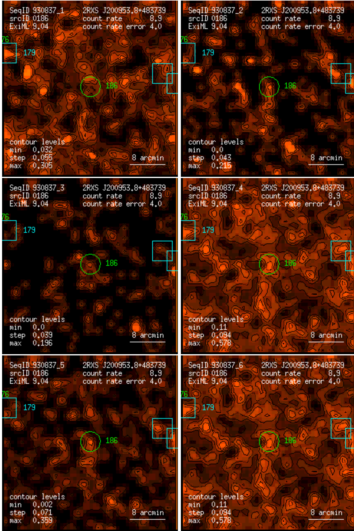
Figure 186: RASS 930837: detection 0186: band rate images, Gaussian filter: (1) PSPC channels 11 – 41, (2) 52 – 90, (3) 91 – 201, (4) 11 – 235, (5) 52 – 201, (6) 11 – 201. Broad band rates in counts/ks. Band rate contour levels in counts/ks/arcmin 2 .
