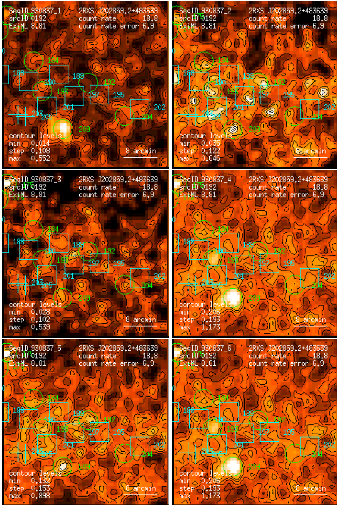
Figure 192: RASS 930837: detection 0192: band rate images, Gaussian filter: (1) PSPC channels 11 – 41, (2) 52 – 90, (3) 91 – 201, (4) 11 – 235, (5) 52 – 201, (6) 11 – 201. Broad band rates in counts/ks. Band rate contour levels in counts/ks/arcmin 2 .
