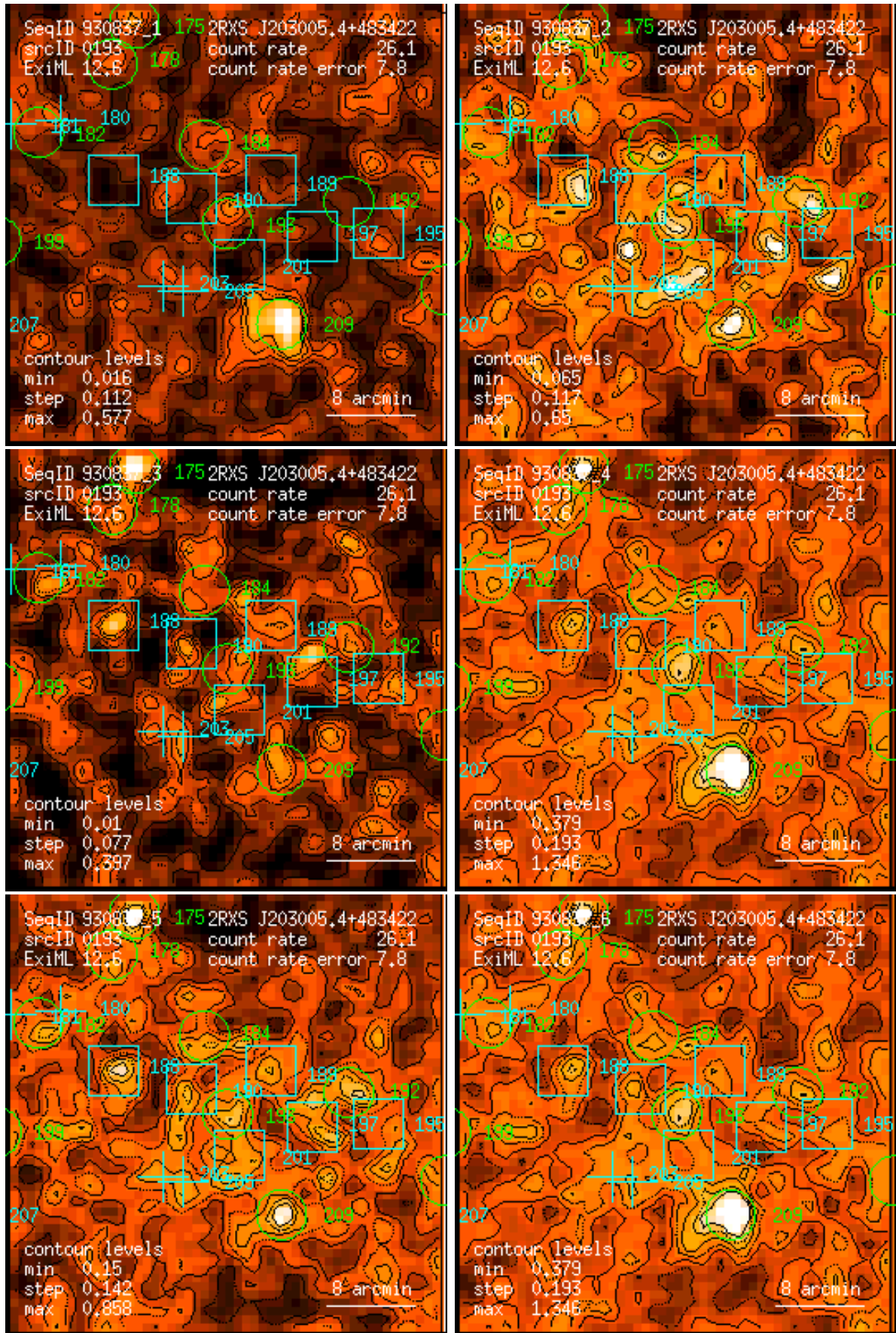
Figure 193: RASS 930837: detection 0193: band rate images, Gaussian filter: (1) PSPC channels 11 – 41, (2) 52 – 90, (3) 91 – 201, (4) 11 – 235, (5) 52 – 201, (6) 11 – 201. Broad band rates in counts/ks. Band rate contour levels in counts/ks/arcmin 2 .
