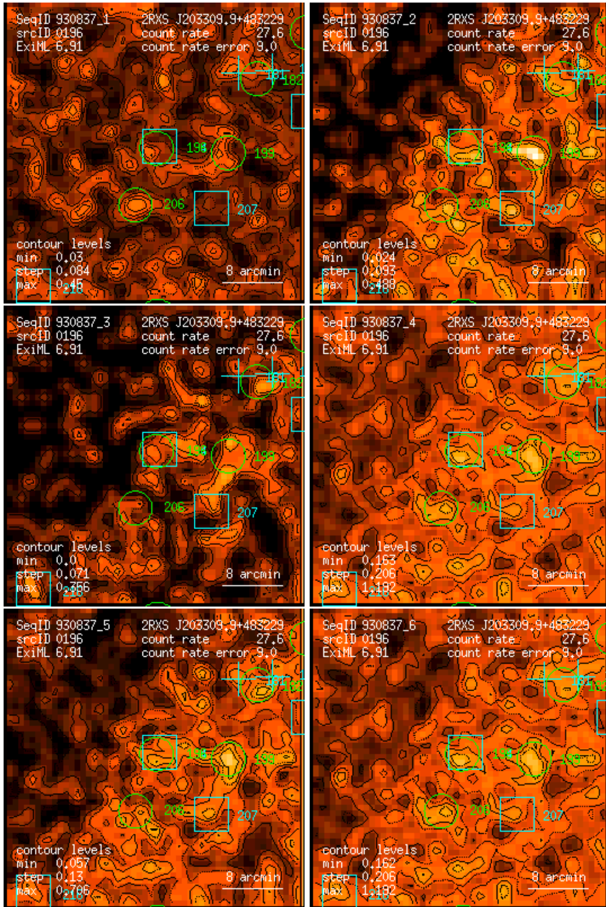
Figure 196: RASS 930837: detection 0196: band rate images, Gaussian filter: (1) PSPC channels 11 – 41, (2) 52 – 90, (3) 91 – 201, (4) 11 – 235, (5) 52 – 201, (6) 11 – 201. Broad band rates in counts/ks. Band rate contour levels in counts/ks/arcmin 2 .
