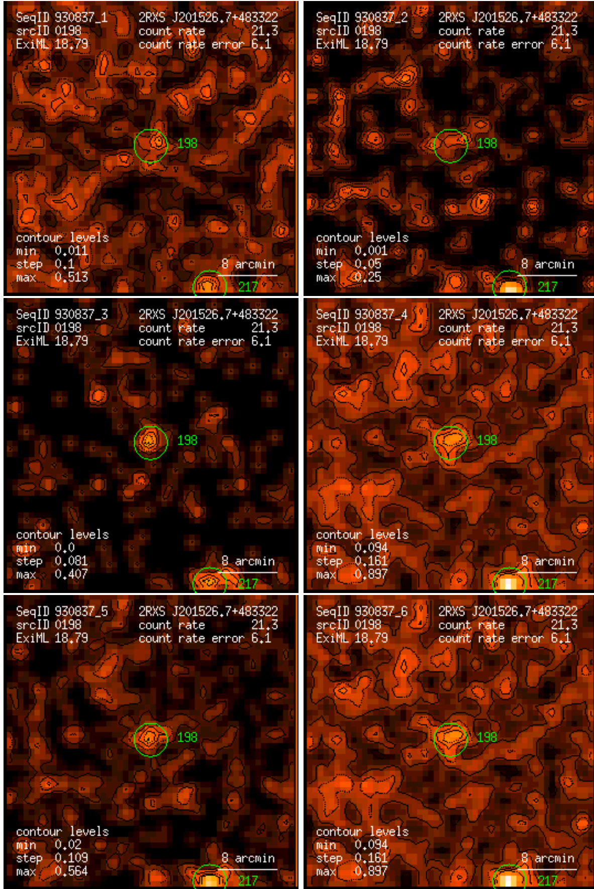
Figure 198: RASS 930837: detection 0198: band rate images, Gaussian filter: (1) PSPC channels 11 – 41, (2) 52 – 90, (3) 91 – 201, (4) 11 – 235, (5) 52 – 201, (6) 11 – 201. Broad band rates in counts/ks. Band rate contour levels in counts/ks/arcmin 2 .
