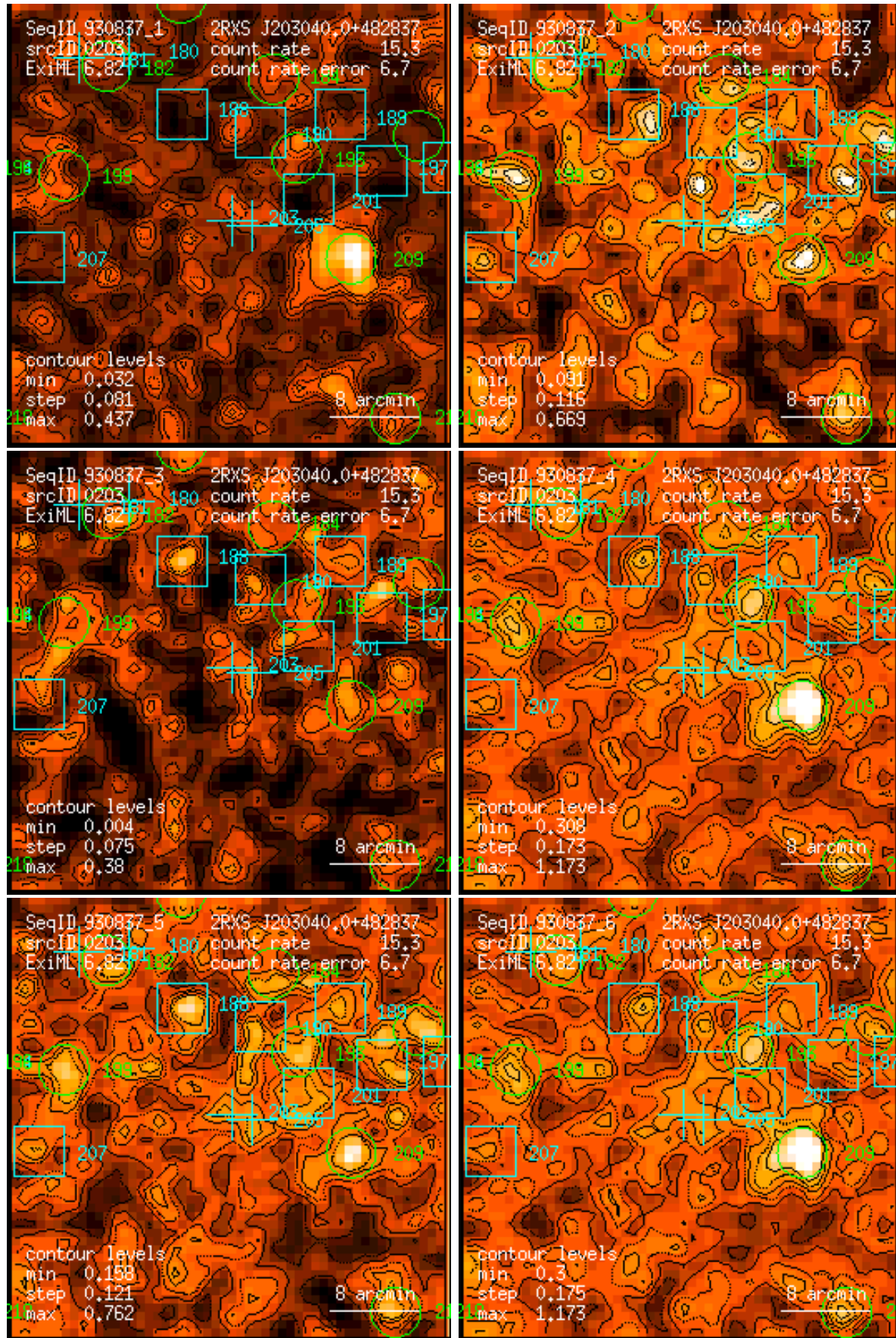
Figure 203: RASS 930837: detection 0203: band rate images, Gaussian filter: (1) PSPC channels 11 – 41, (2) 52 – 90, (3) 91 – 201, (4) 11 – 235, (5) 52 – 201, (6) 11 – 201. Broad band rates in counts/ks. Band rate contour levels in counts/ks/arcmin 2 .
