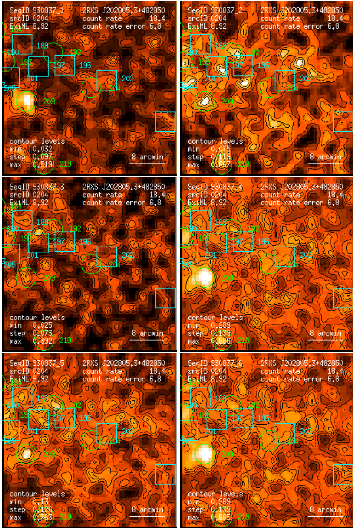
Figure 204: RASS 930837: detection 0204: band rate images, Gaussian filter: (1) PSPC channels 11 – 41, (2) 52 – 90, (3) 91 – 201, (4) 11 – 235, (5) 52 – 201, (6) 11 – 201. Broad band rates in counts/ks. Band rate contour levels in counts/ks/arcmin 2 .
