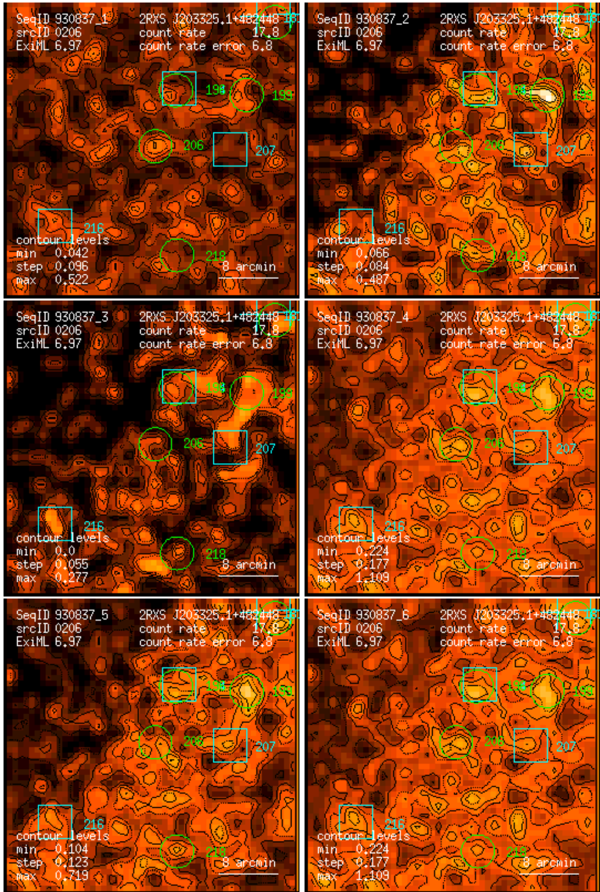
Figure 206: RASS 930837: detection 0206: band rate images, Gaussian filter: (1) PSPC channels 11 – 41, (2) 52 – 90, (3) 91 – 201, (4) 11 – 235, (5) 52 – 201, (6) 11 – 201. Broad band rates in counts/ks. Band rate contour levels in counts/ks/arcmin 2 .
