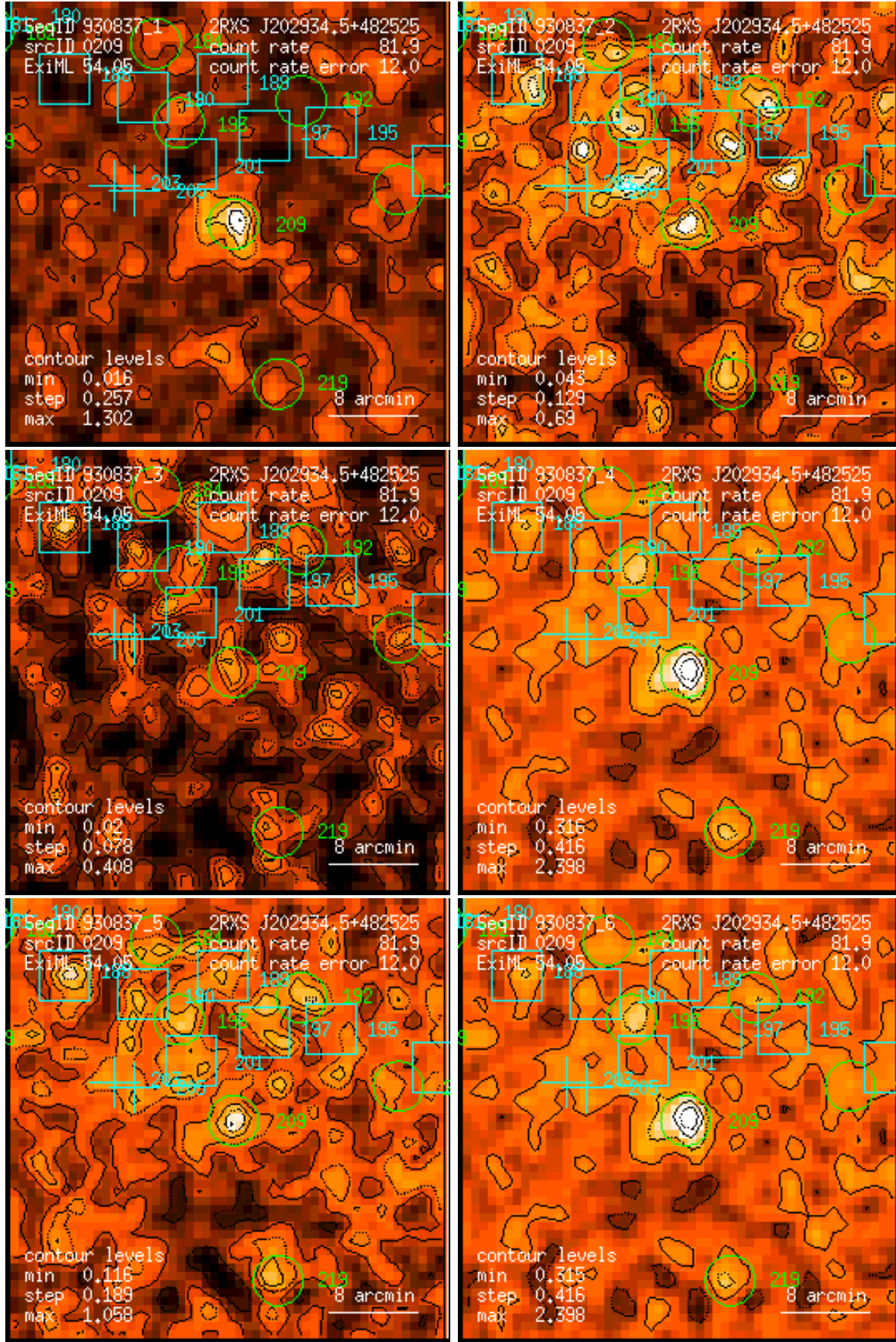
Figure 209: RASS 930837: detection 0209: band rate images, Gaussian filter: (1) PSPC channels 11 – 41, (2) 52 – 90, (3) 91 – 201, (4) 11 – 235, (5) 52 – 201, (6) 11 – 201. Broad band rates in counts/ks. Band rate contour levels in counts/ks/arcmin 2 .
