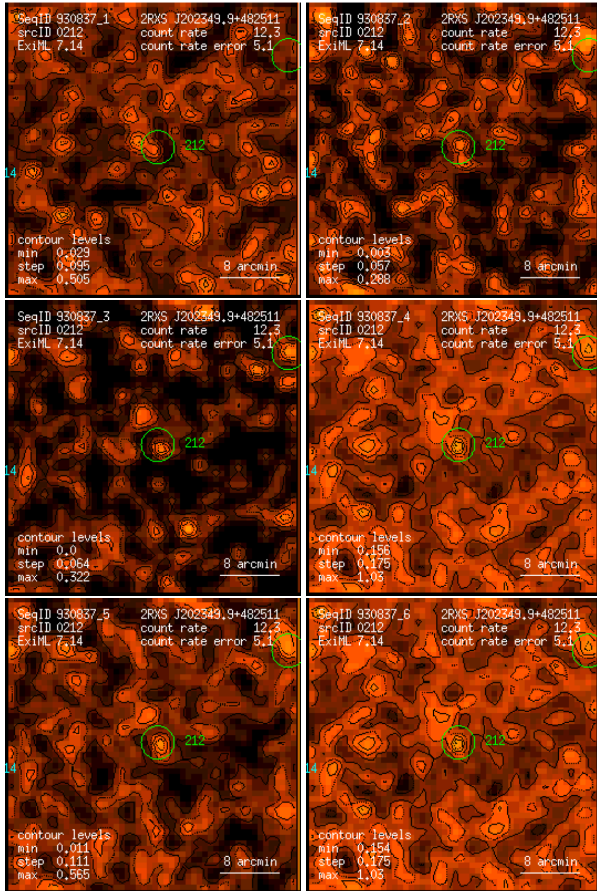
Figure 212: RASS 930837: detection 0212: band rate images, Gaussian filter: (1) PSPC channels 11 – 41, (2) 52 – 90, (3) 91 – 201, (4) 11 – 235, (5) 52 – 201, (6) 11 – 201. Broad band rates in counts/ks. Band rate contour levels in counts/ks/arcmin 2 .
