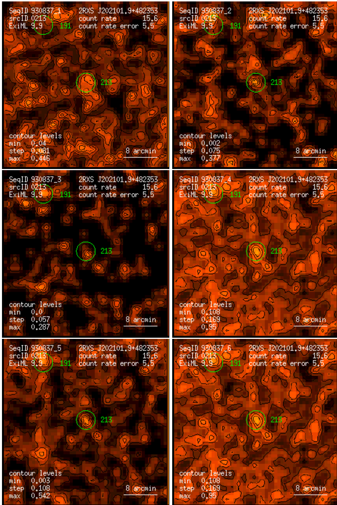
Figure 213: RASS 930837: detection 0213: band rate images, Gaussian filter: (1) PSPC channels 11 – 41, (2) 52 – 90, (3) 91 – 201, (4) 11 – 235, (5) 52 – 201, (6) 11 – 201. Broad band rates in counts/ks. Band rate contour levels in counts/ks/arcmin 2 .
