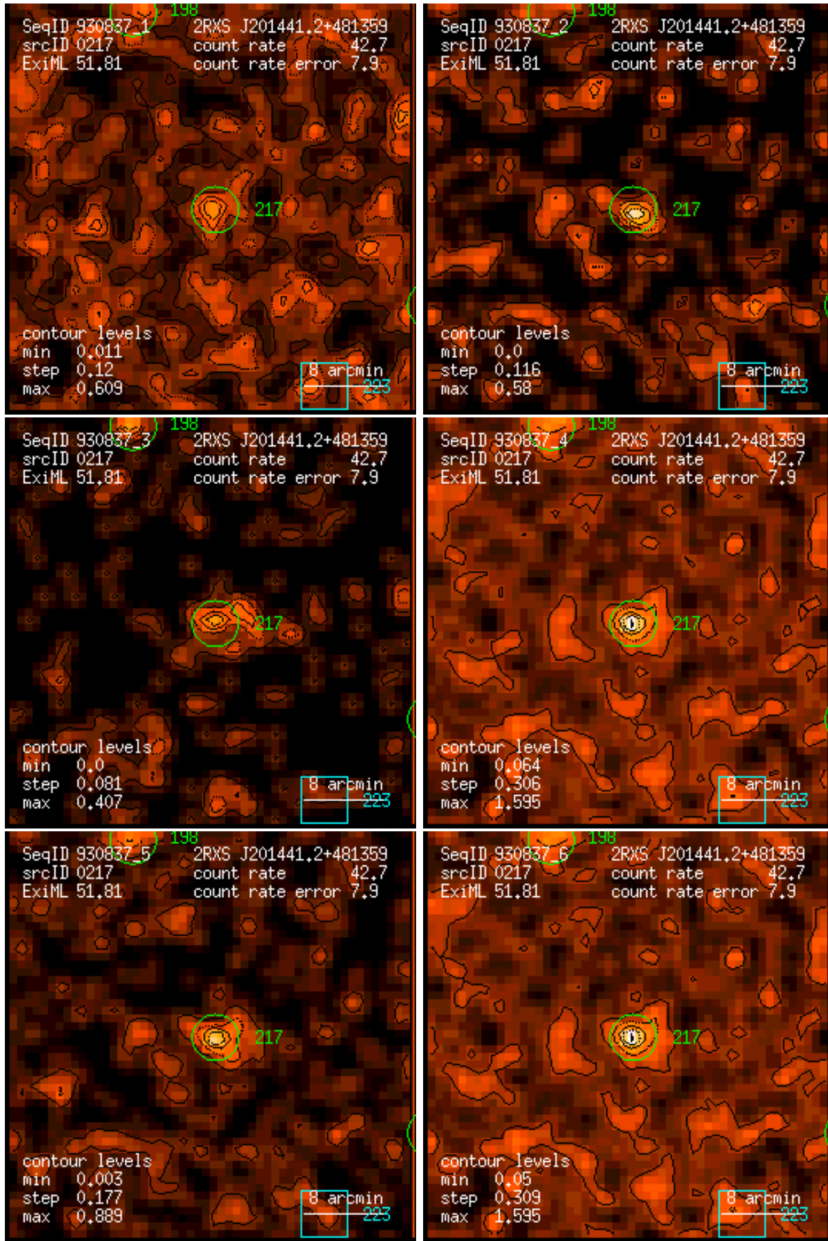
Figure 217: RASS 930837: detection 0217: band rate images, Gaussian filter: (1) PSPC channels 11 – 41, (2) 52 – 90, (3) 91 – 201, (4) 11 – 235, (5) 52 – 201, (6) 11 – 201. Broad band rates in counts/ks. Band rate contour levels in counts/ks/arcmin 2 .
