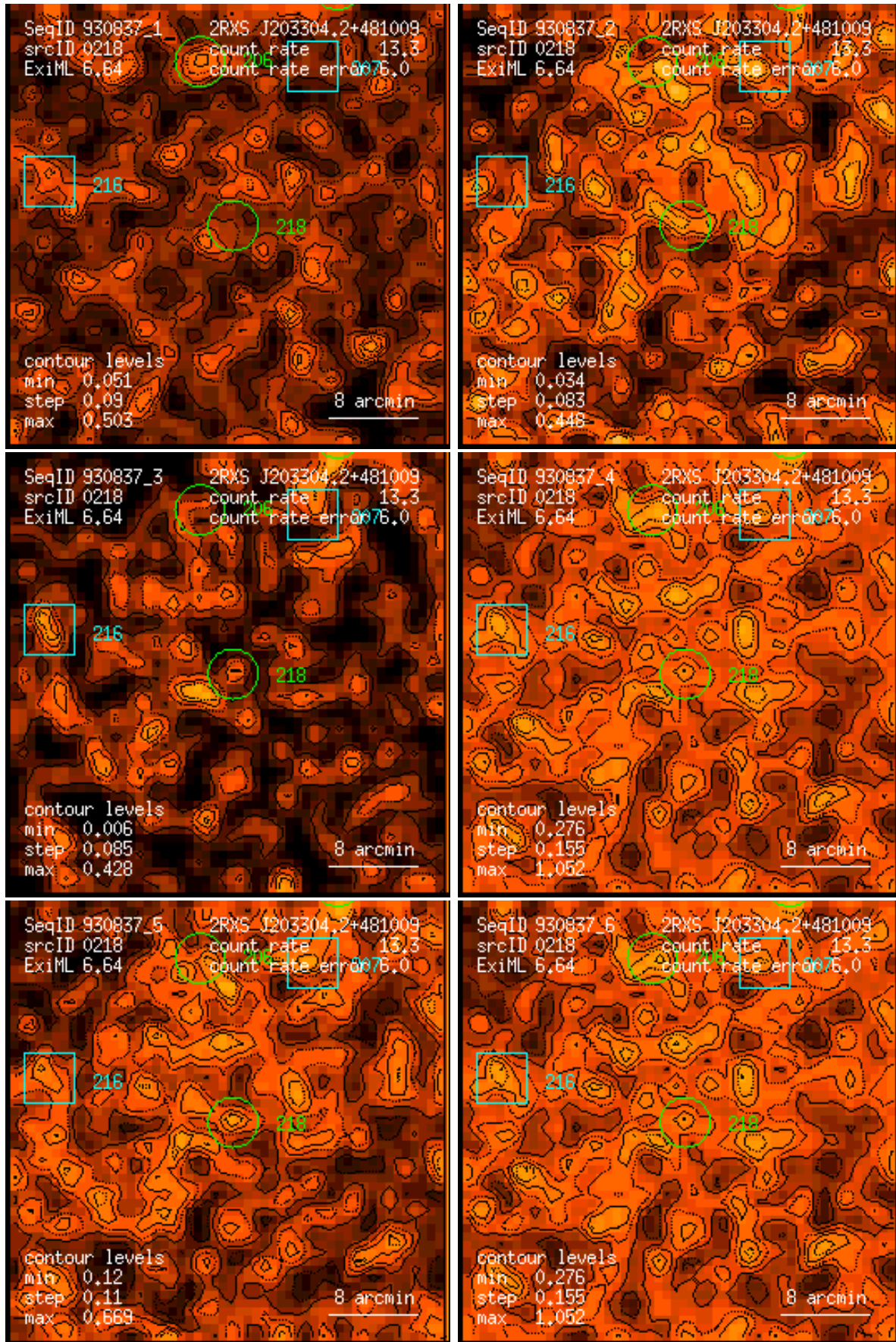
Figure 218: RASS 930837: detection 0218: band rate images, Gaussian filter: (1) PSPC channels 11 – 41, (2) 52 – 90, (3) 91 – 201, (4) 11 – 235, (5) 52 – 201, (6) 11 – 201. Broad band rates in counts/ks. Band rate contour levels in counts/ks/arcmin 2 .
