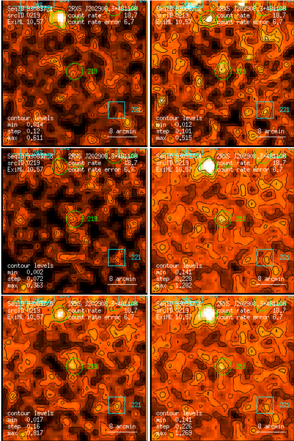
Figure 219: RASS 930837: detection 0219: band rate images, Gaussian filter: (1) PSPC channels 11 – 41, (2) 52 – 90, (3) 91 – 201, (4) 11 – 235, (5) 52 – 201, (6) 11 – 201. Broad band rates in counts/ks. Band rate contour levels in counts/ks/arcmin 2 .
