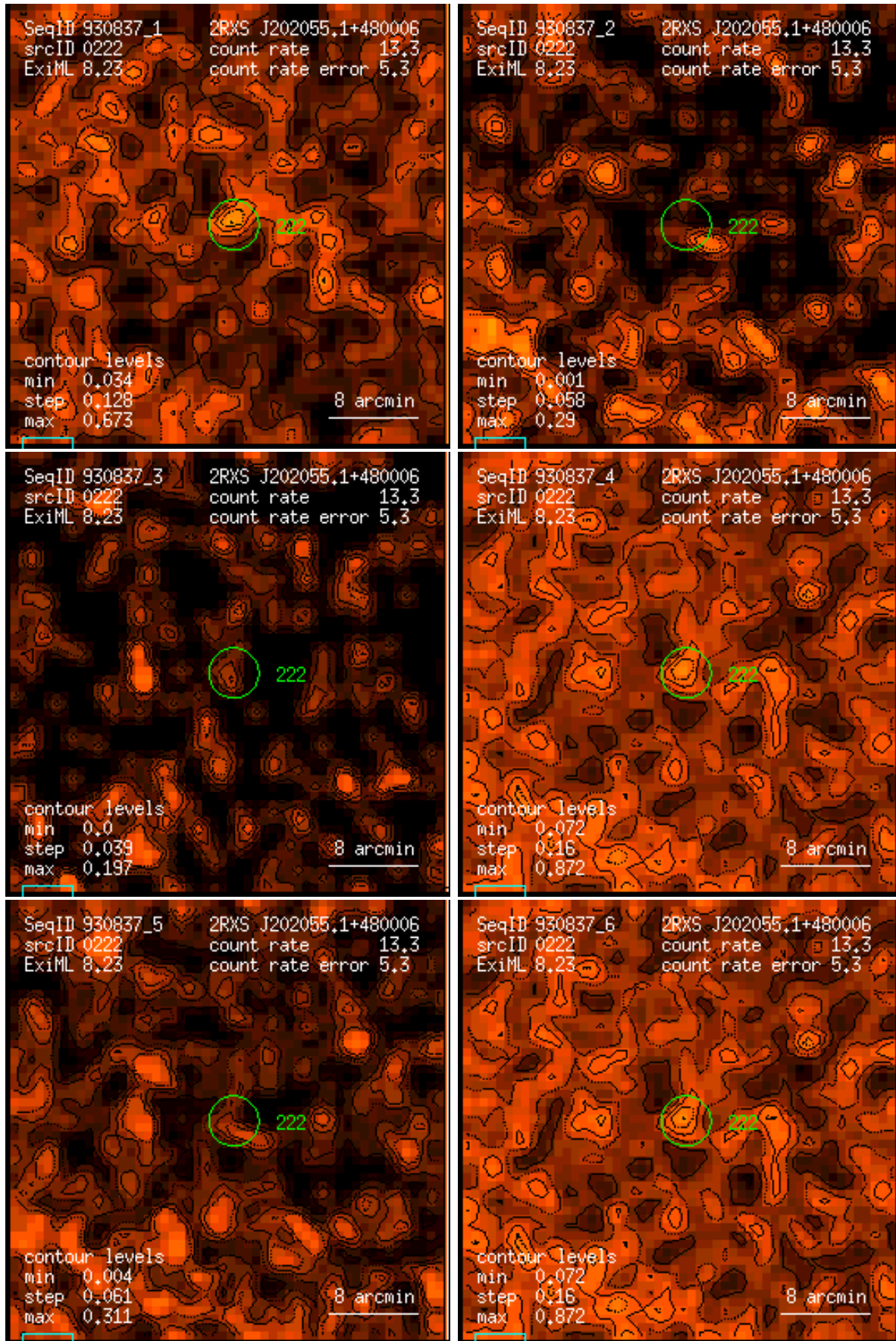
Figure 222: RASS 930837: detection 0222: band rate images, Gaussian filter: (1) PSPC channels 11 – 41, (2) 52 – 90, (3) 91 – 201, (4) 11 – 235, (5) 52 – 201, (6) 11 – 201. Broad band rates in counts/ks. Band rate contour levels in counts/ks/arcmin 2 .
