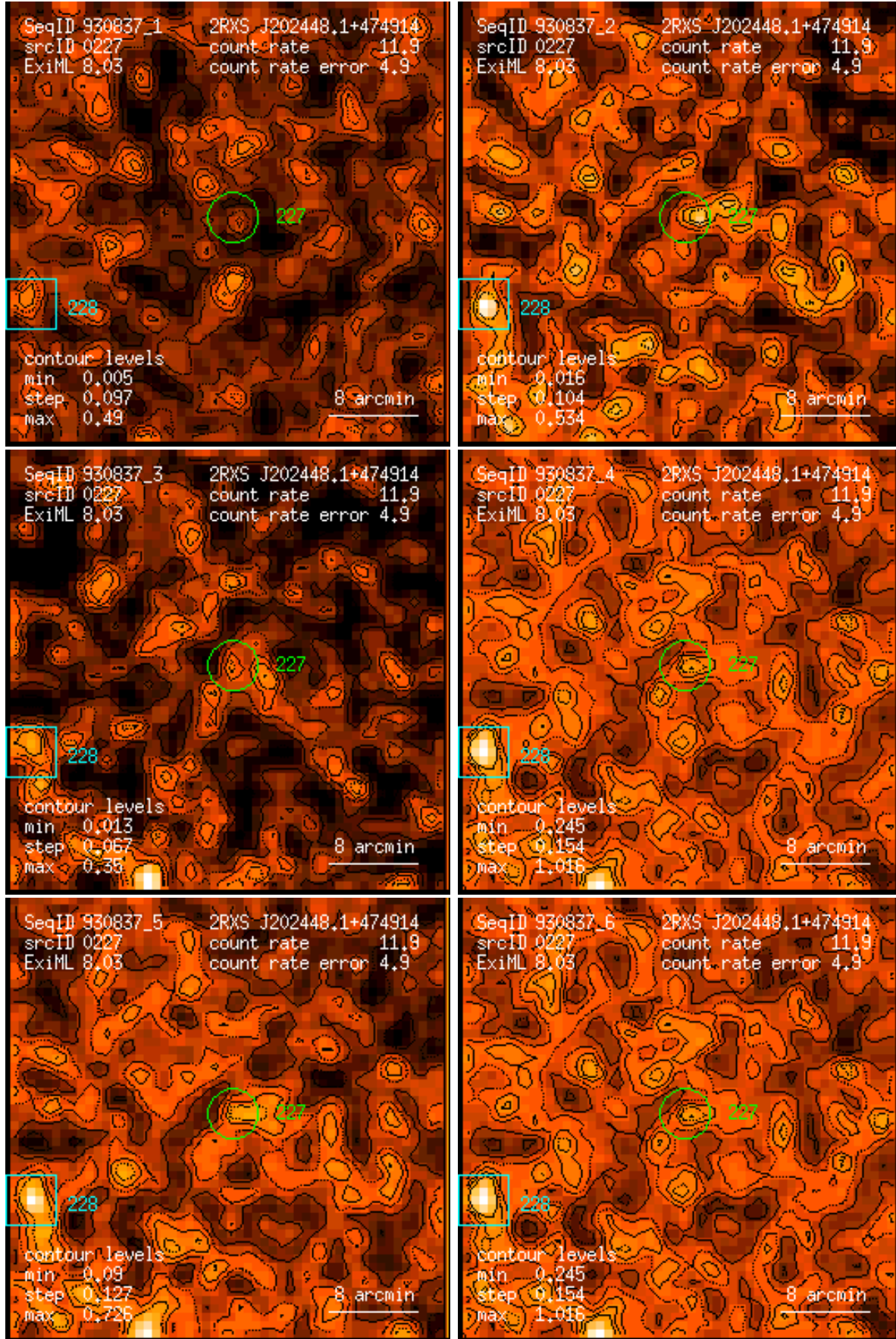
Figure 227: RASS 930837: detection 0227: band rate images, Gaussian filter: (1) PSPC channels 11 – 41, (2) 52 – 90, (3) 91 – 201, (4) 11 – 235, (5) 52 – 201, (6) 11 – 201. Broad band rates in counts/ks. Band rate contour levels in counts/ks/arcmin 2 .
