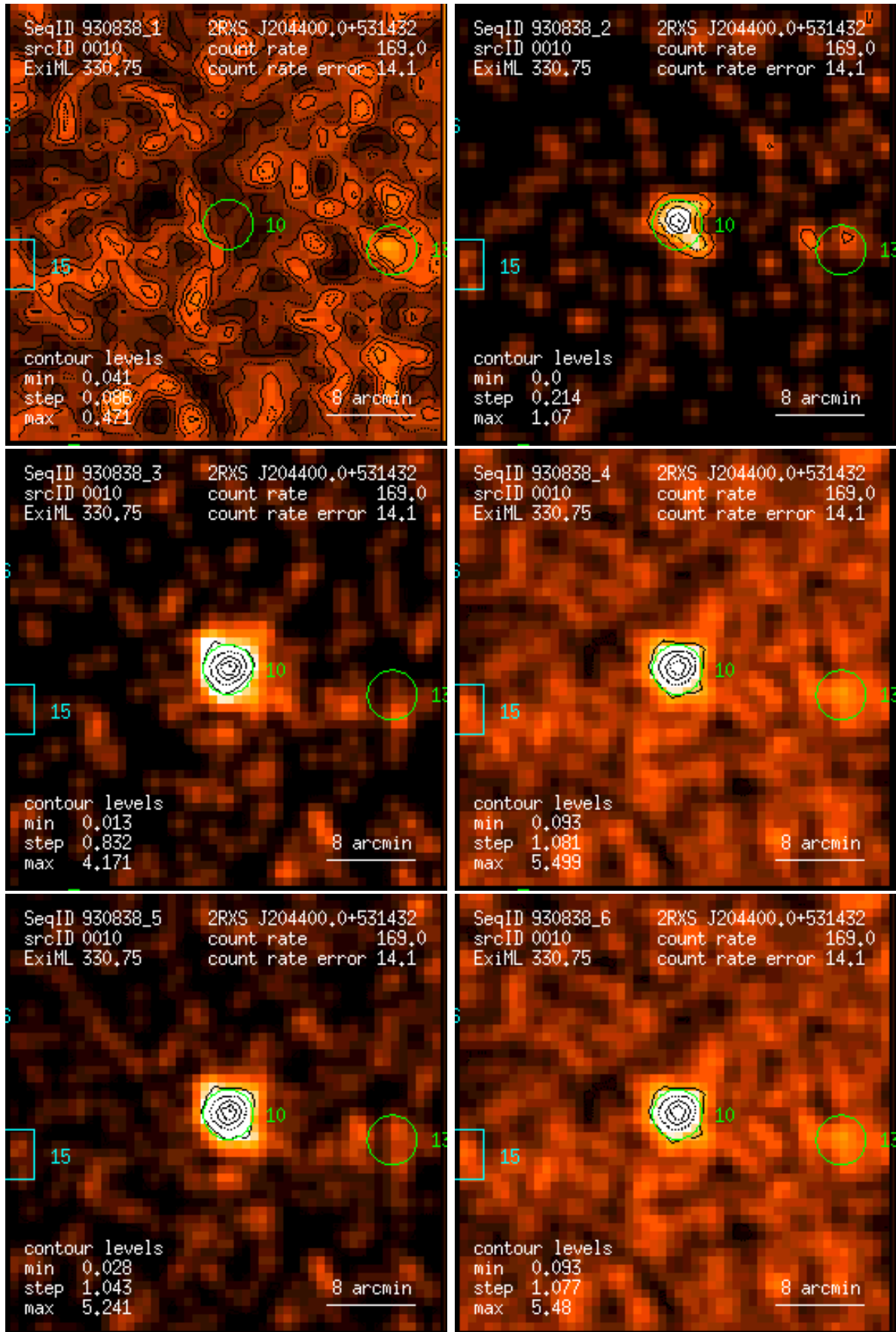
Figure 10: RASS 930838: detection 0010: band rate images, Gaussian filter: (1) PSPC channels 11 – 41, (2) 52 – 90, (3) 91 – 201, (4) 11 – 235, (5) 52 – 201, (6) 11 – 201. Broad band rates in counts/ks. Band rate contour levels in counts/ks/arcmin 2 .
