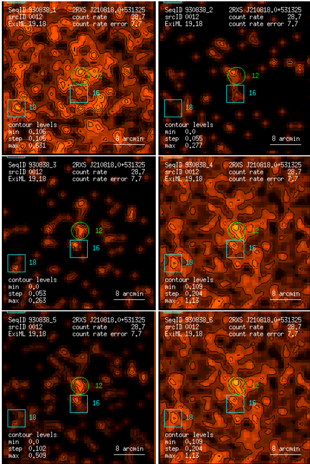
Figure 12: RASS 930838: detection 0012: band rate images, Gaussian filter: (1) PSPC channels 11 – 41, (2) 52 – 90, (3) 91 – 201, (4) 11 – 235, (5) 52 – 201, (6) 11 – 201. Broad band rates in counts/ks. Band rate contour levels in counts/ks/arcmin 2 .
