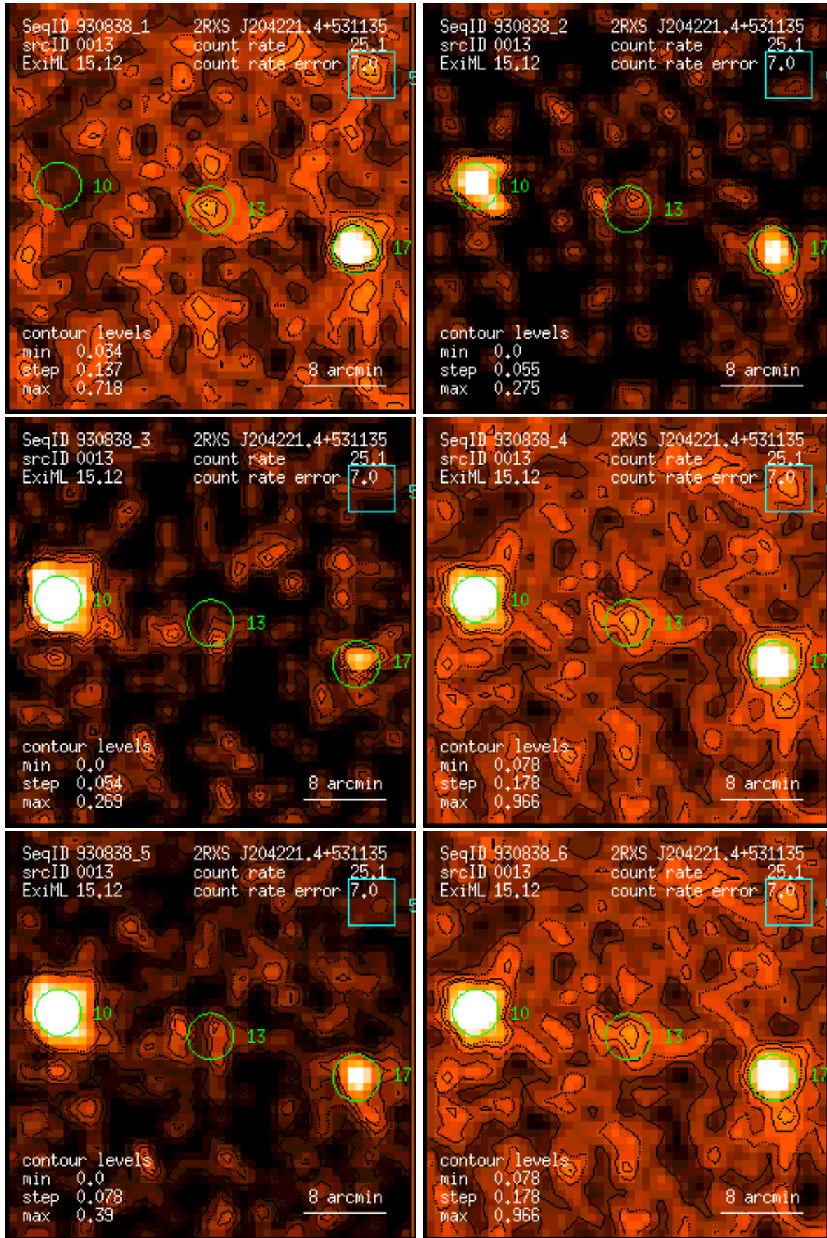
Figure 13: RASS 930838: detection 0013: band rate images, Gaussian filter: (1) PSPC channels 11 – 41, (2) 52 – 90, (3) 91 – 201, (4) 11 – 235, (5) 52 – 201, (6) 11 – 201. Broad band rates in counts/ks. Band rate contour levels in counts/ks/arcmin 2 .
