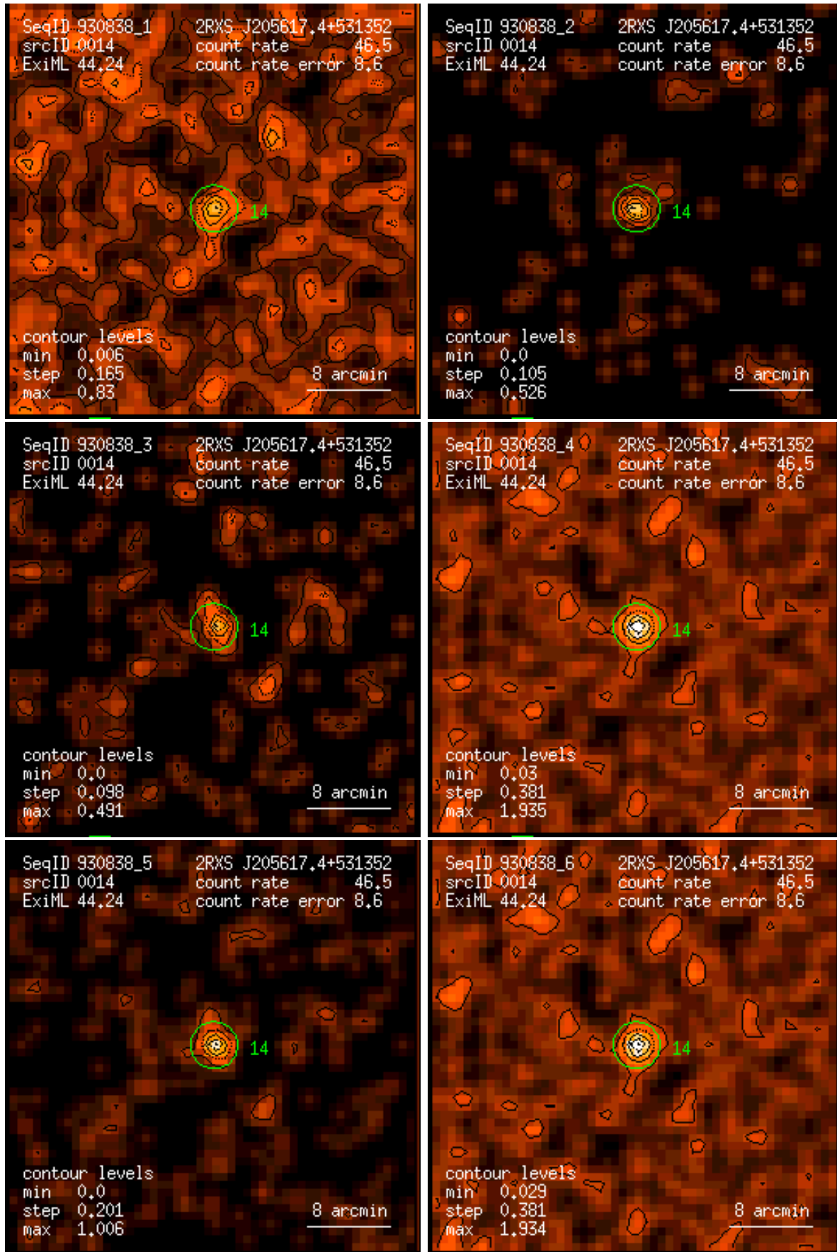
Figure 14: RASS 930838: detection 0014: band rate images, Gaussian filter: (1) PSPC channels 11 – 41, (2) 52 – 90, (3) 91 – 201, (4) 11 – 235, (5) 52 – 201, (6) 11 – 201. Broad band rates in counts/ks. Band rate contour levels in counts/ks/arcmin 2 .
