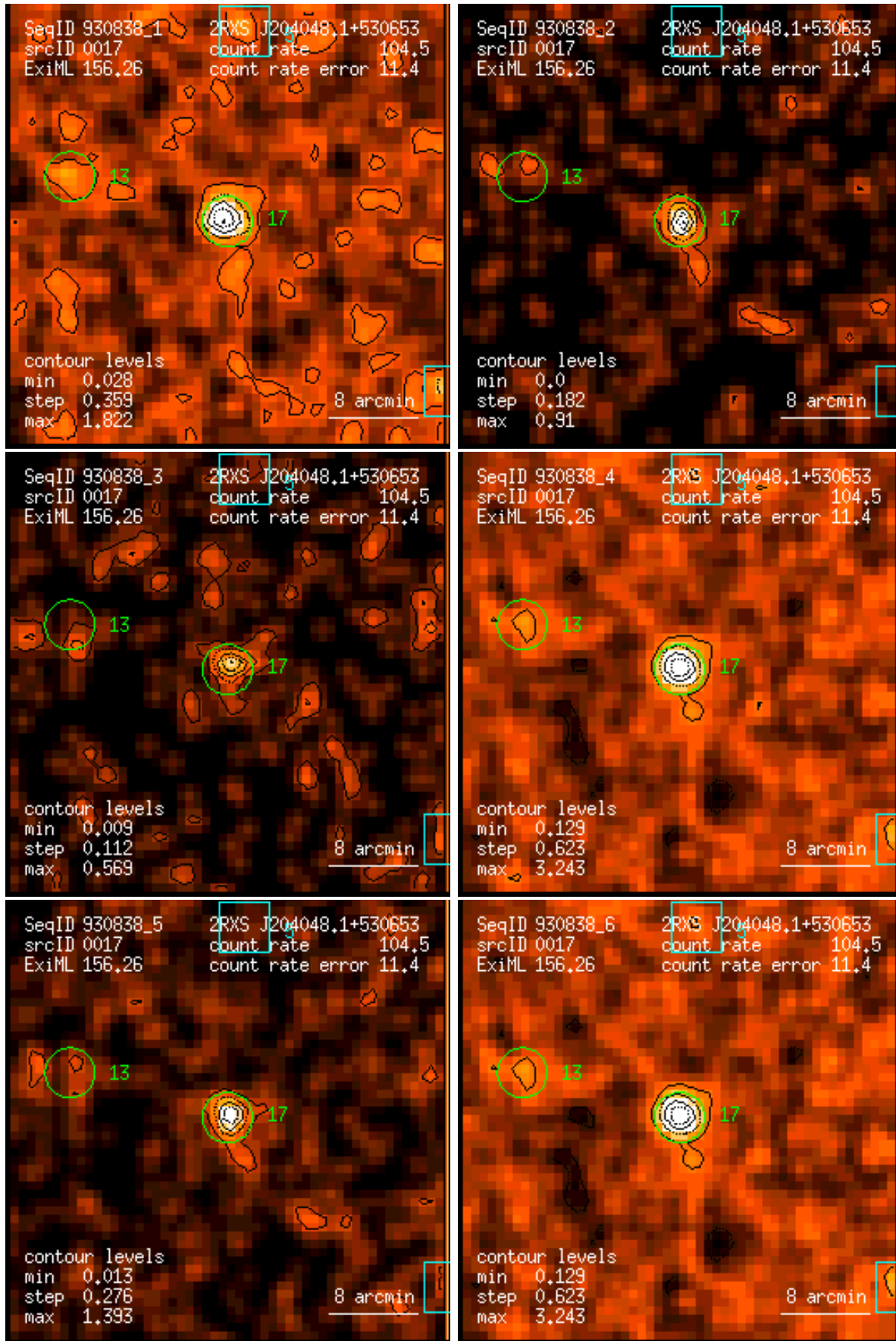
Figure 17: RASS 930838: detection 0017: band rate images, Gaussian filter: (1) PSPC channels 11 – 41, (2) 52 – 90, (3) 91 – 201, (4) 11 – 235, (5) 52 – 201, (6) 11 – 201. Broad band rates in counts/ks. Band rate contour levels in counts/ks/arcmin 2 .
