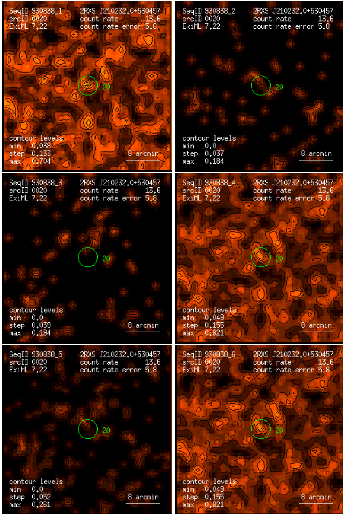
Figure 20: RASS 930838: detection 0020: band rate images, Gaussian filter: (1) PSPC channels 11 – 41, (2) 52 – 90, (3) 91 – 201, (4) 11 – 235, (5) 52 – 201, (6) 11 – 201. Broad band rates in counts/ks. Band rate contour levels in counts/ks/arcmin 2 .
