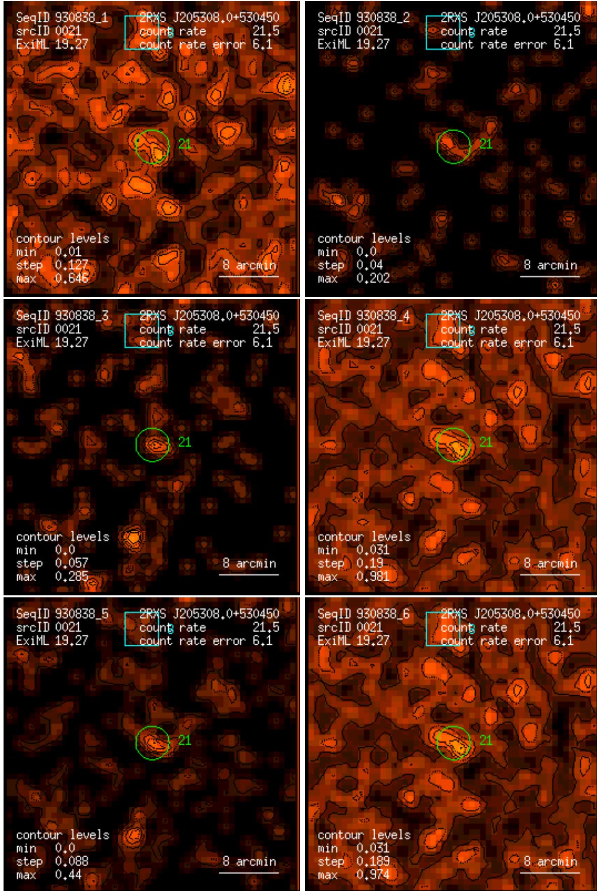
Figure 21: RASS 930838: detection 0021: band rate images, Gaussian filter: (1) PSPC channels 11 – 41, (2) 52 – 90, (3) 91 – 201, (4) 11 – 235, (5) 52 – 201, (6) 11 – 201. Broad band rates in counts/ks. Band rate contour levels in counts/ks/arcmin 2 .
