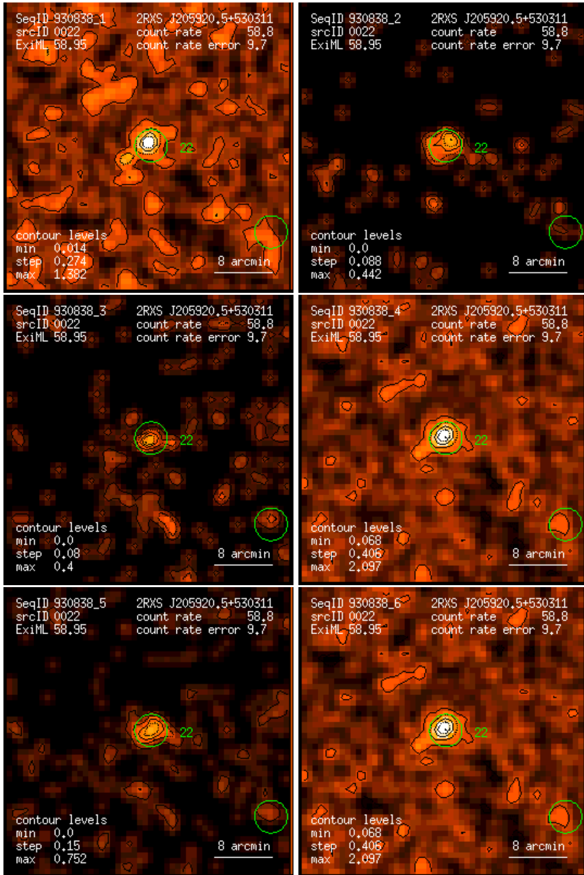
Figure 22: RASS 930838: detection 0022: band rate images, Gaussian filter: (1) PSPC channels 11 – 41, (2) 52 – 90, (3) 91 – 201, (4) 11 – 235, (5) 52 – 201, (6) 11 – 201. Broad band rates in counts/ks. Band rate contour levels in counts/ks/arcmin 2 .
