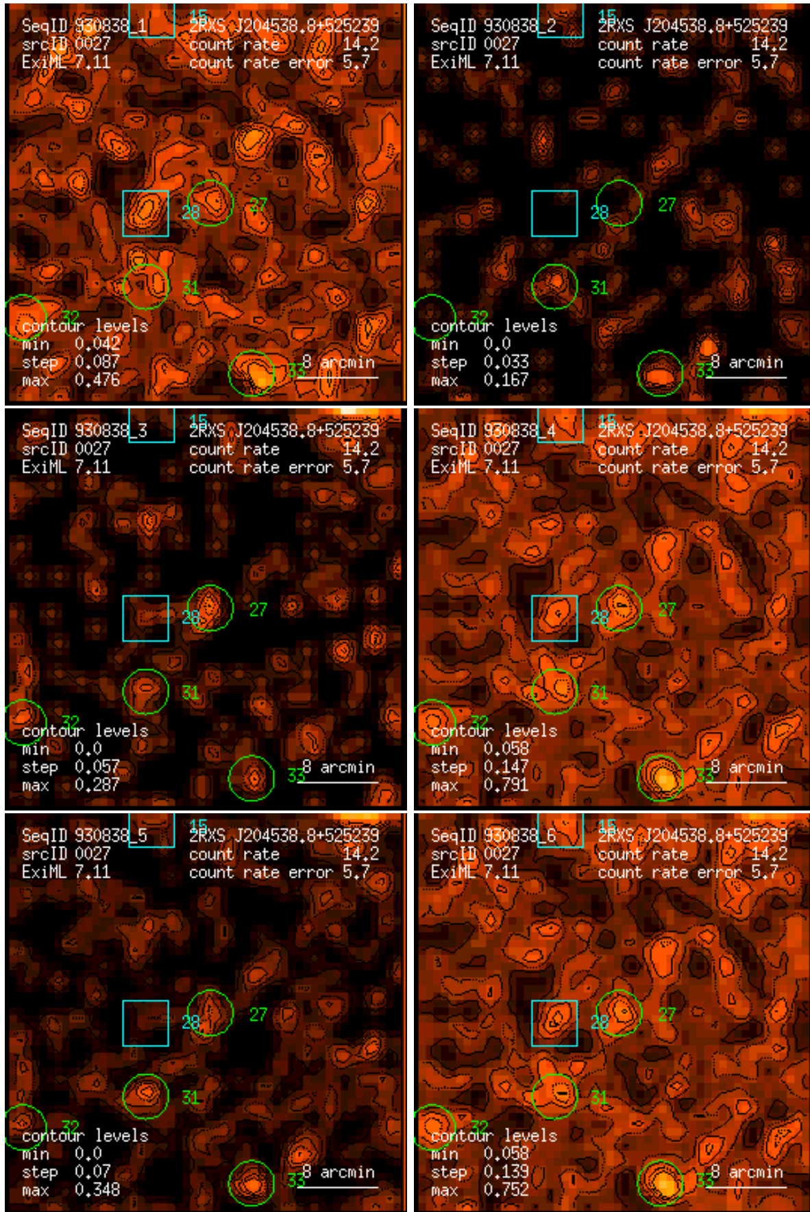
Figure 27: RASS 930838: detection 0027: band rate images, Gaussian filter: (1) PSPC channels 11 – 41, (2) 52 – 90, (3) 91 – 201, (4) 11 – 235, (5) 52 – 201, (6) 11 – 201. Broad band rates in counts/ks. Band rate contour levels in counts/ks/arcmin 2 .
