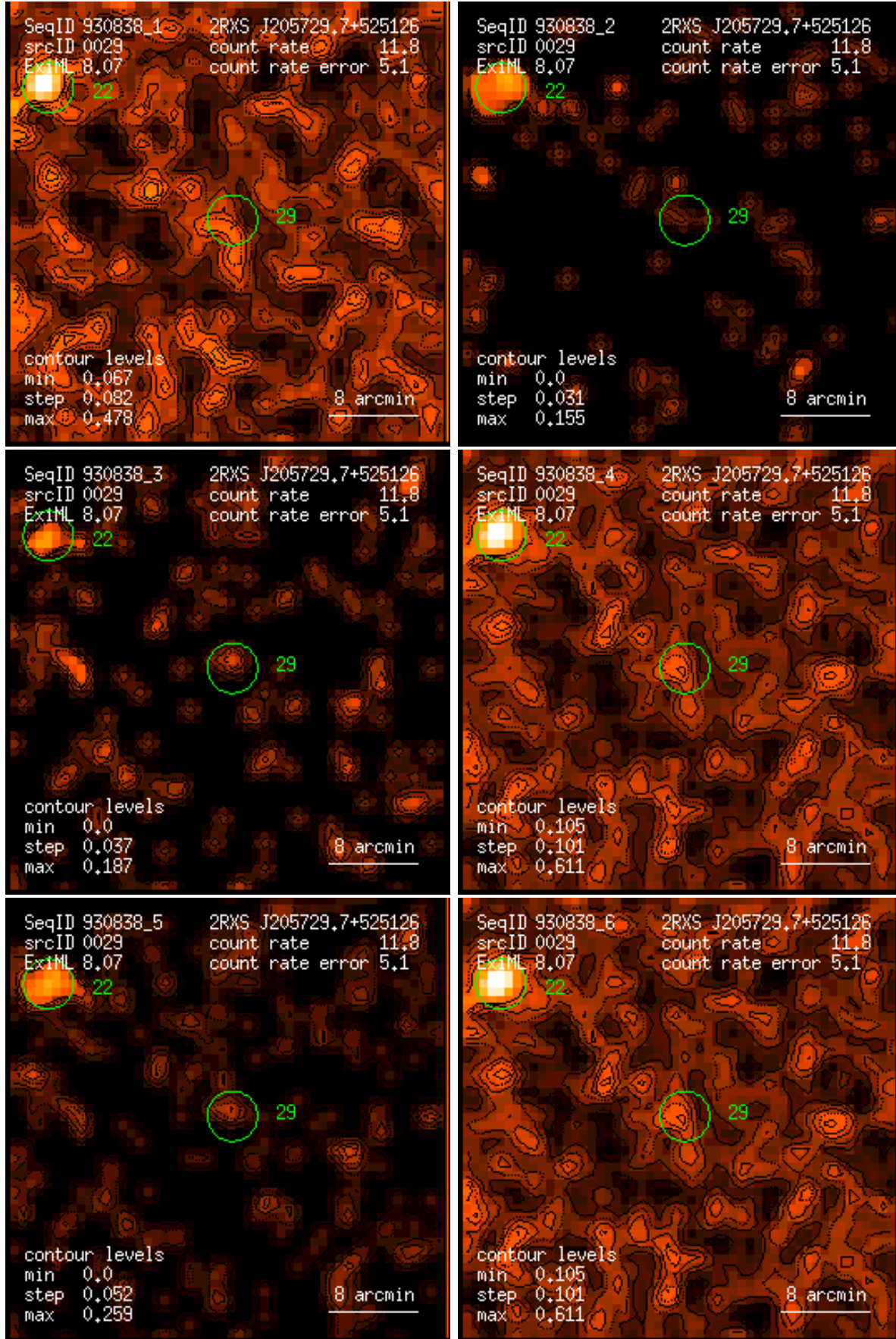
Figure 29: RASS 930838: detection 0029: band rate images, Gaussian filter: (1) PSPC channels 11 – 41, (2) 52 – 90, (3) 91 – 201, (4) 11 – 235, (5) 52 – 201, (6) 11 – 201. Broad band rates in counts/ks. Band rate contour levels in counts/ks/arcmin 2 .
