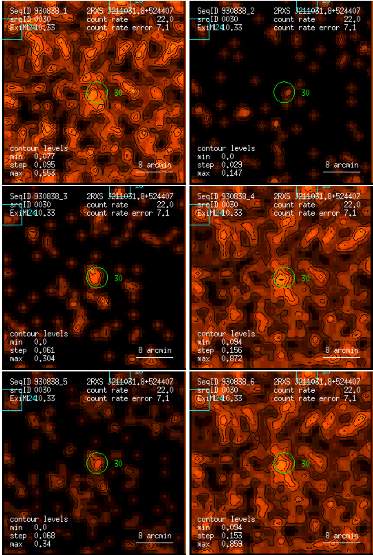
Figure 30: RASS 930838: detection 0030: band rate images, Gaussian filter: (1) PSPC channels 11 – 41, (2) 52 – 90, (3) 91 – 201, (4) 11 – 235, (5) 52 – 201, (6) 11 – 201. Broad band rates in counts/ks. Band rate contour levels in counts/ks/arcmin 2 .
