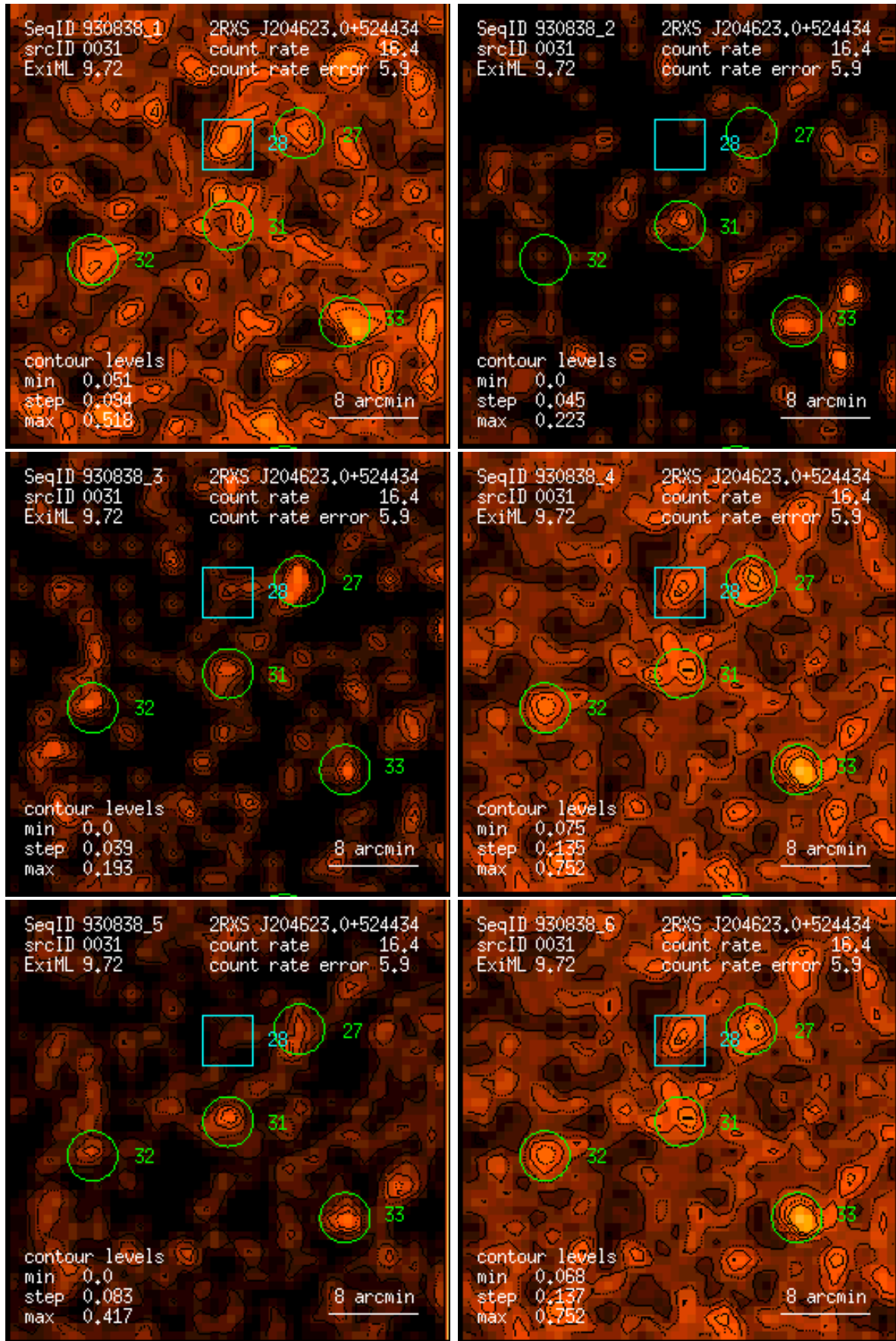
Figure 31: RASS 930838: detection 0031: band rate images, Gaussian filter: (1) PSPC channels 11 – 41, (2) 52 – 90, (3) 91 – 201, (4) 11 – 235, (5) 52 – 201, (6) 11 – 201. Broad band rates in counts/ks. Band rate contour levels in counts/ks/arcmin 2 .
