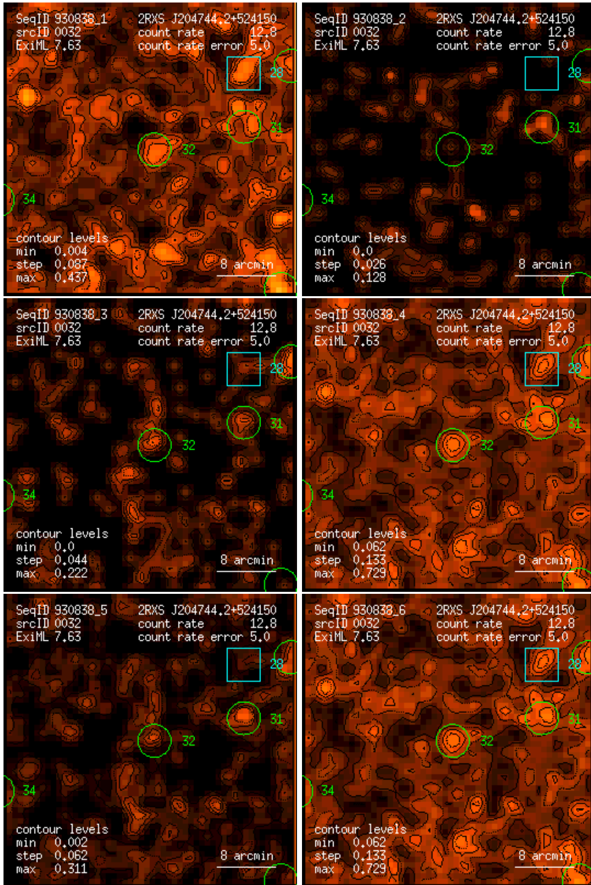
Figure 32: RASS 930838: detection 0032: band rate images, Gaussian filter: (1) PSPC channels 11 – 41, (2) 52 – 90, (3) 91 – 201, (4) 11 – 235, (5) 52 – 201, (6) 11 – 201. Broad band rates in counts/ks. Band rate contour levels in counts/ks/arcmin 2 .
