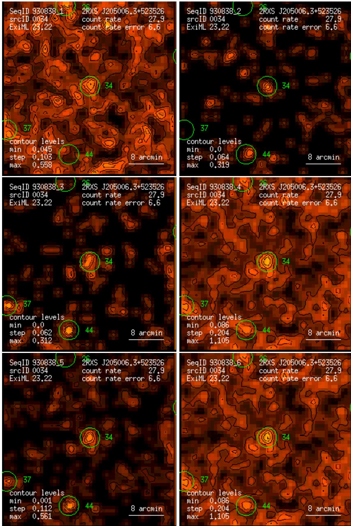
Figure 34: RASS 930838: detection 0034: band rate images, Gaussian filter: (1) PSPC channels 11 – 41, (2) 52 – 90, (3) 91 – 201, (4) 11 – 235, (5) 52 – 201, (6) 11 – 201. Broad band rates in counts/ks. Band rate contour levels in counts/ks/arcmin 2 .
