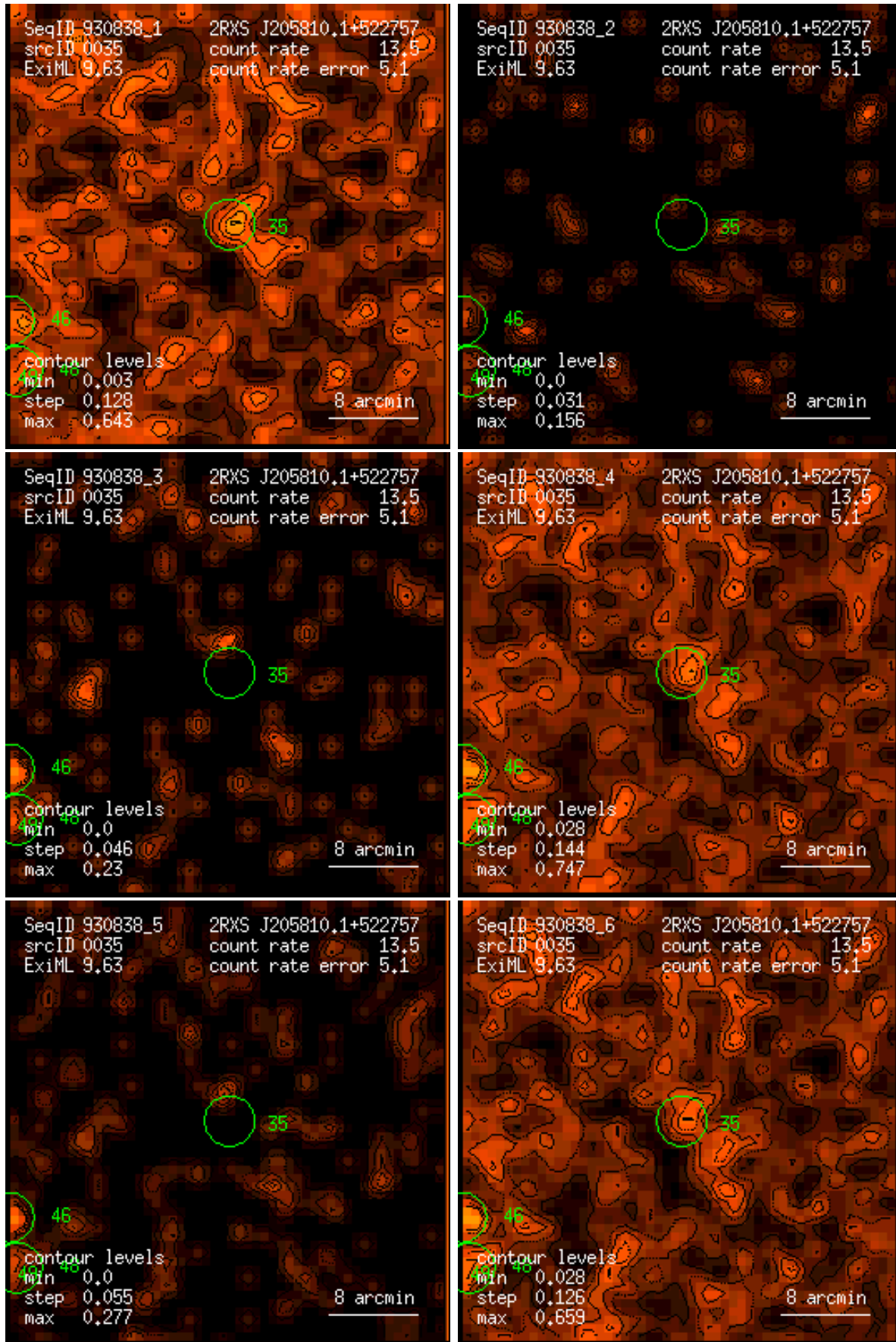
Figure 35: RASS 930838: detection 0035: band rate images, Gaussian filter: (1) PSPC channels 11 – 41, (2) 52 – 90, (3) 91 – 201, (4) 11 – 235, (5) 52 – 201, (6) 11 – 201. Broad band rates in counts/ks. Band rate contour levels in counts/ks/arcmin 2 .
