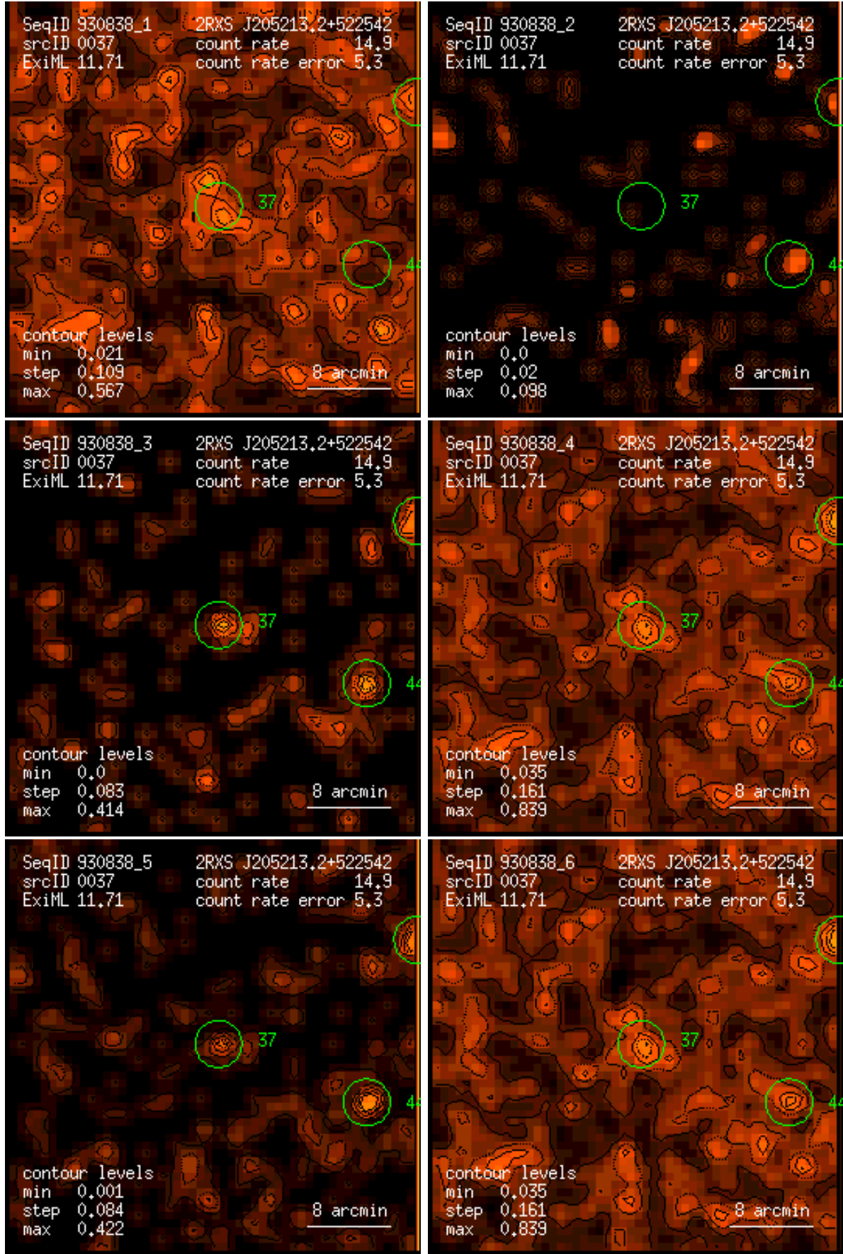
Figure 37: RASS 930838: detection 0037: band rate images, Gaussian filter: (1) PSPC channels 11 – 41, (2) 52 – 90, (3) 91 – 201, (4) 11 – 235, (5) 52 – 201, (6) 11 – 201. Broad band rates in counts/ks. Band rate contour levels in counts/ks/arcmin 2 .
