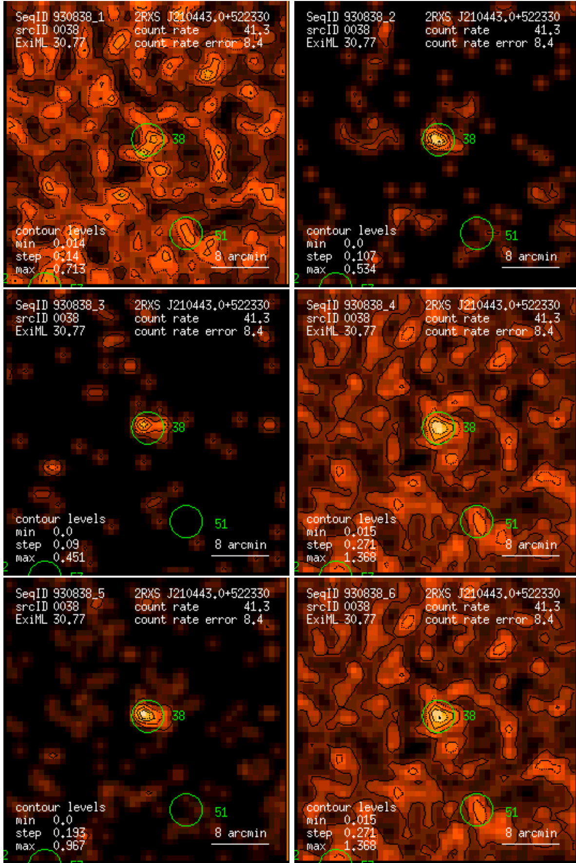
Figure 38: RASS 930838: detection 0038: band rate images, Gaussian filter: (1) PSPC channels 11 – 41, (2) 52 – 90, (3) 91 – 201, (4) 11 – 235, (5) 52 – 201, (6) 11 – 201. Broad band rates in counts/ks. Band rate contour levels in counts/ks/arcmin 2 .
