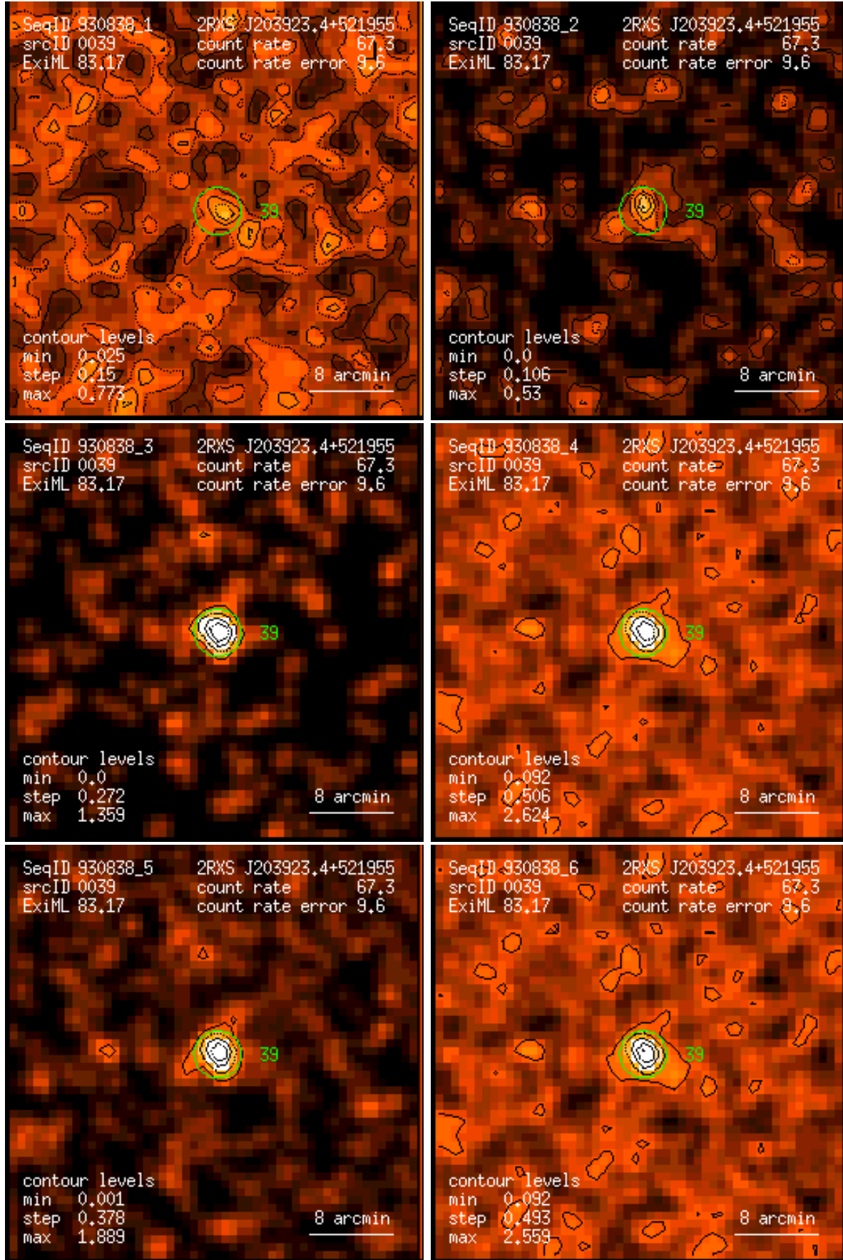
Figure 39: RASS 930838: detection 0039: band rate images, Gaussian filter: (1) PSPC channels 11 – 41, (2) 52 – 90, (3) 91 – 201, (4) 11 – 235, (5) 52 – 201, (6) 11 – 201. Broad band rates in counts/ks. Band rate contour levels in counts/ks/arcmin 2 .
