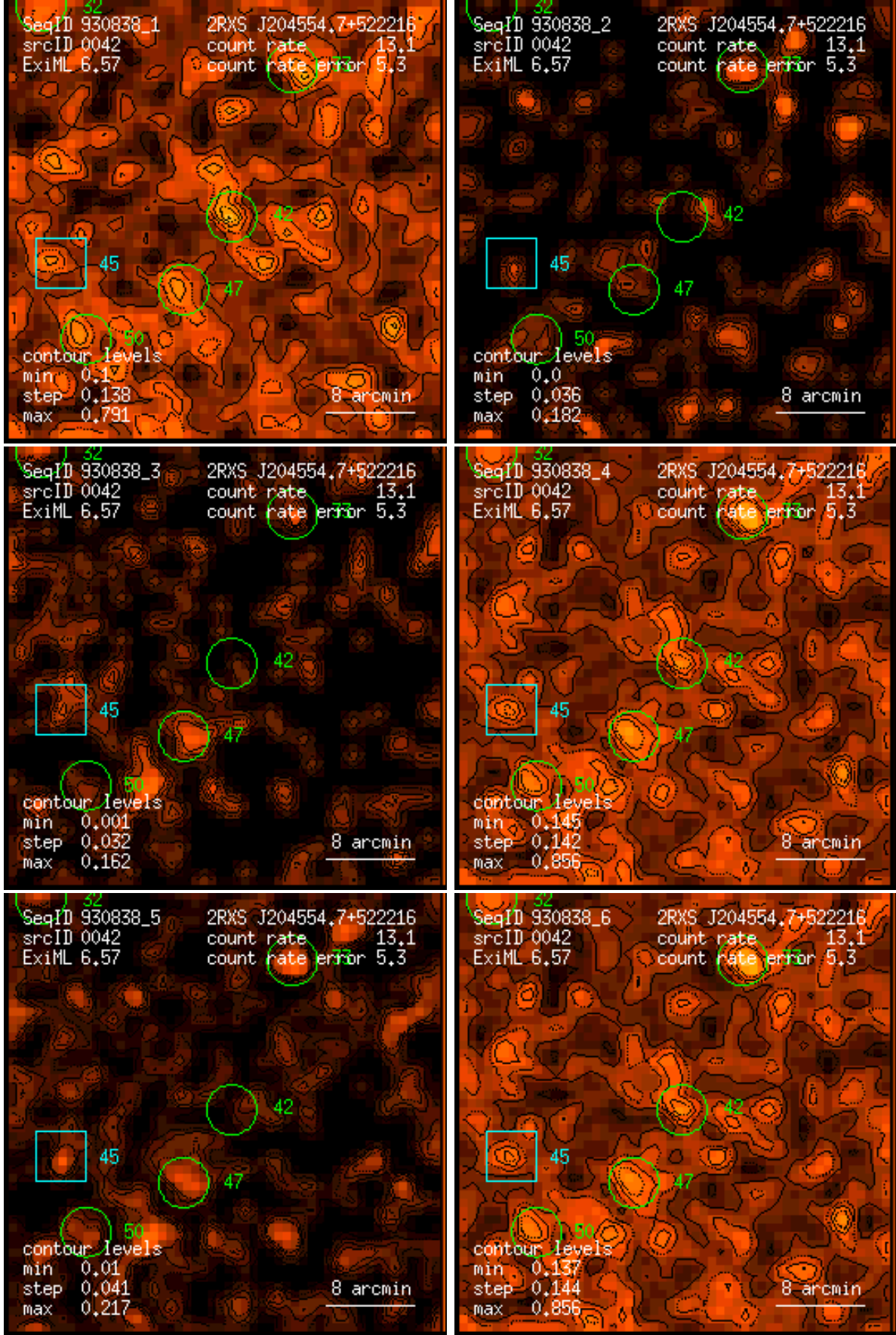
Figure 42: RASS 930838: detection 0042: band rate images, Gaussian filter: (1) PSPC channels 11 – 41, (2) 52 – 90, (3) 91 – 201, (4) 11 – 235, (5) 52 – 201, (6) 11 – 201. Broad band rates in counts/ks. Band rate contour levels in counts/ks/arcmin 2 .
