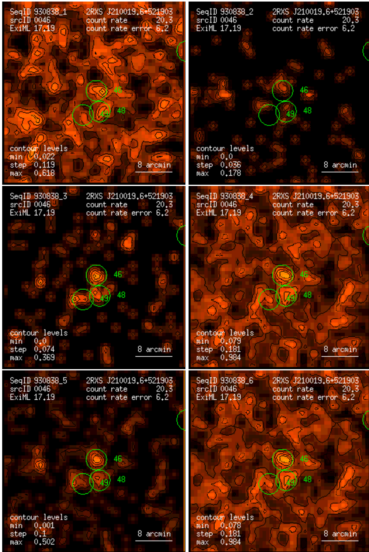
Figure 46: RASS 930838: detection 0046: band rate images, Gaussian filter: (1) PSPC channels 11 – 41, (2) 52 – 90, (3) 91 – 201, (4) 11 – 235, (5) 52 – 201, (6) 11 – 201. Broad band rates in counts/ks. Band rate contour levels in counts/ks/arcmin 2 .
